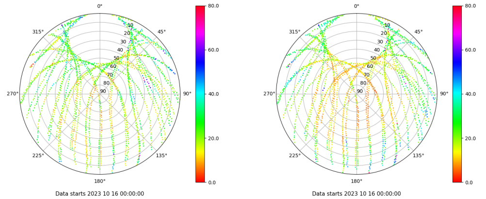
Skyplot for station VALE. Parameter M1C Data file VALE00ESP_R_2023289.xtr Skyplot for station VALE. Parameter M2P Data file VALE00ESP_R_2023289.xtr
