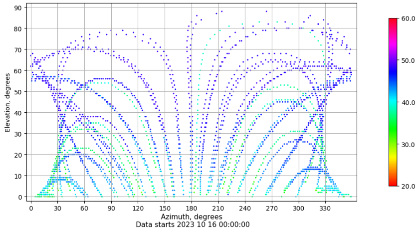
Azimuth-elevation plot for station VALE. Signal to Noise S1C Data file VALE00ESP_R_2023289.xtr
