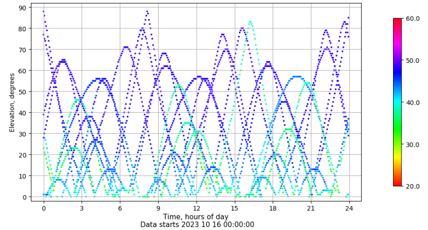
Time-elevation plot for station VALE. Signal to Noise S1C Data file VALE00ESP_R_2023289.xtr
