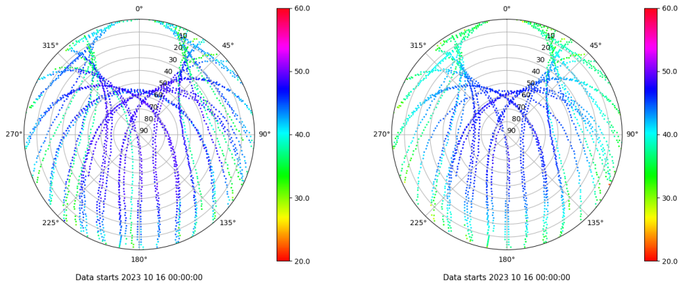
Skyplot for station VALE. Signal to Noise S1C Data file VALE00ESP_R_2023289.xtr Skyplot for station VALE. Signal to Noise S2P Data file VALE00ESP_R_2023289.xtr
