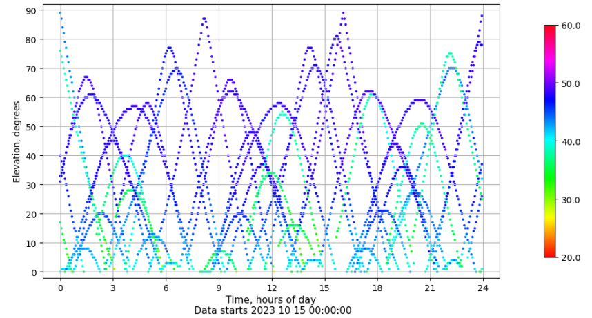
Time-elevation plot for station VALE. Signal to Noise S1C Data file VALE00ESP_R_2023288.xtr
