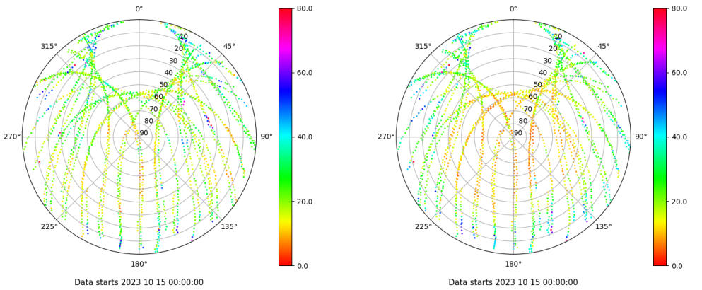
Skyplot for station VALE. Parameter M1C Data file VALE00ESP_R_2023288.xtr Skyplot for station VALE. Parameter M2P Data file VALE00ESP_R_2023288.xtr
