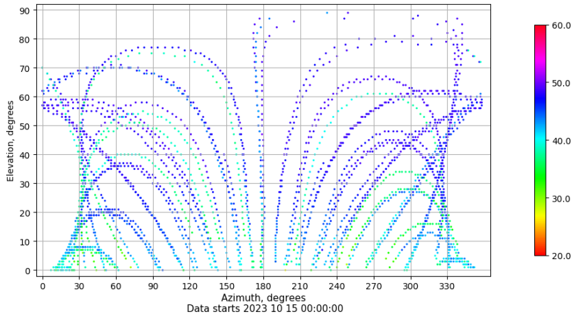
Azimuth-elevation plot for station VALE. Signal to Noise S1C Data file VALE00ESP_R_2023288.xtr
