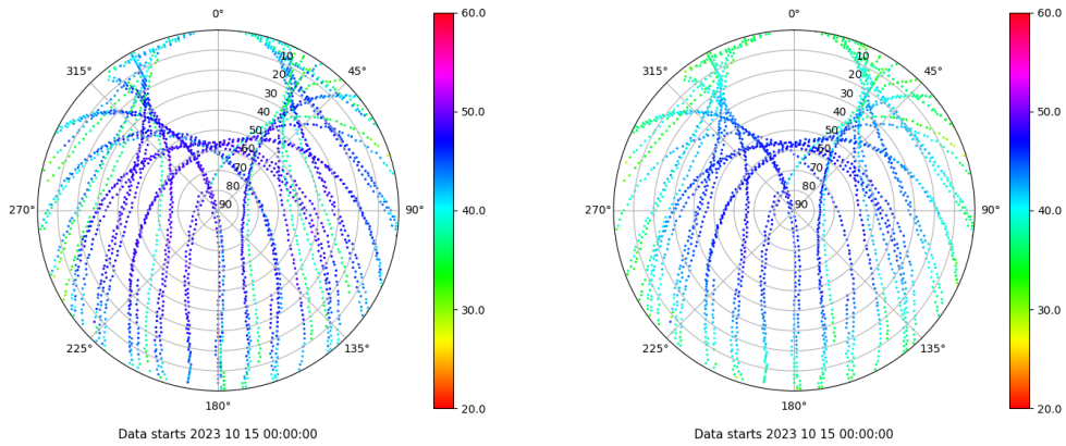
Skyplot for station VALE. Signal to Noise S1C Data file VALE00ESP_R_2023288.xtr Skyplot for station VALE. Signal to Noise S2P Data file VALE00ESP_R_2023288.xtr
