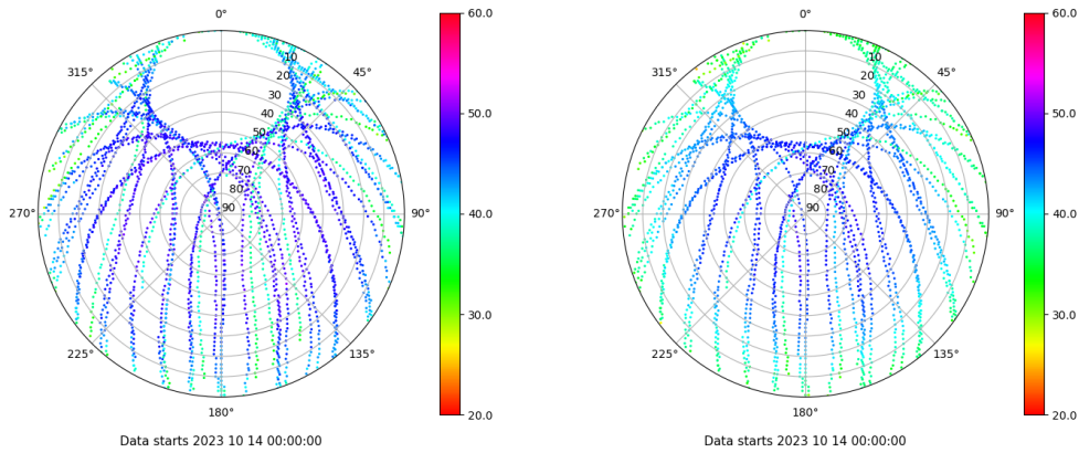
Skyplot for station VALE. Signal to Noise S1C Data file VALE00ESP_R_2023287.xtr Skyplot for station VALE. Signal to Noise S2P Data file VALE00ESP_R_2023287.xtr
