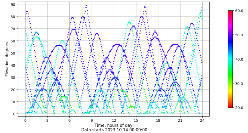
Time-elevation plot for station VALE. Signal to Noise S1C Data file VALE00ESP_R_2023287.xtr
