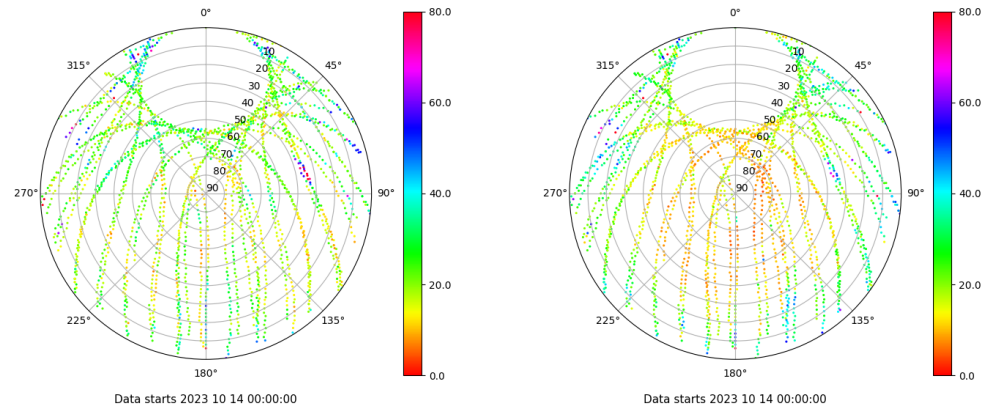
Skyplot for station VALE. Parameter M1C Data file VALE00ESP_R_2023287.xtr Skyplot for station VALE. Parameter M2P Data file VALE00ESP_R_2023287.xtr
