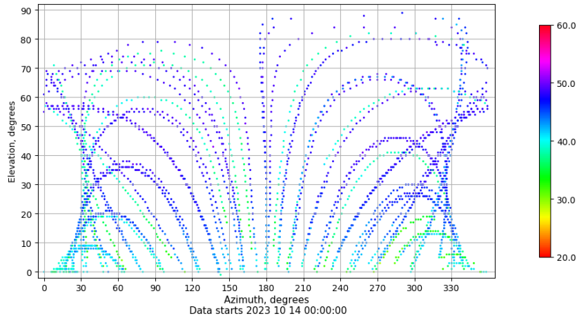
Azimuth-elevation plot for station VALE. Signal to Noise S1C Data file VALE00ESP_R_2023287.xtr
