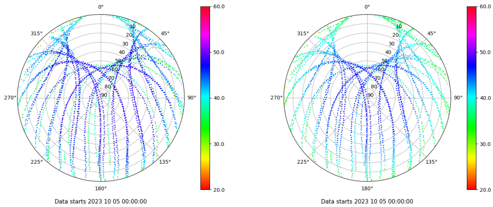
Skyplot for station VALE. Signal to Noise S1C Data file VALE00ESP_R_2023278.xtr Skyplot for station VALE. Signal to Noise S2P Data file VALE00ESP_R_2023278.xtr
