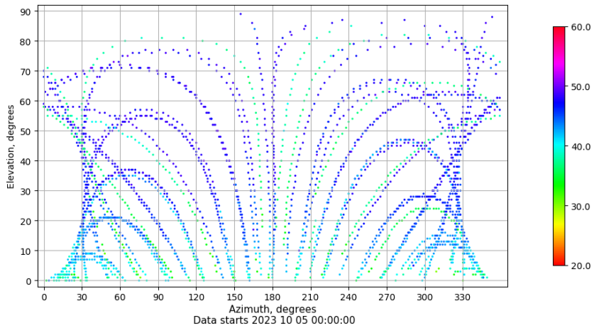
Azimuth-elevation plot for station VALE. Signal to Noise S1C Data file VALE00ESP_R_2023278.xtr
