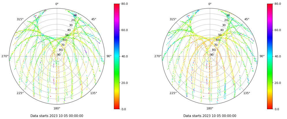
Skyplot for station VALE. Parameter M1C Data file VALE00ESP_R_2023278.xtr Skyplot for station VALE. Parameter M2P Data file VALE00ESP_R_2023278.xtr
