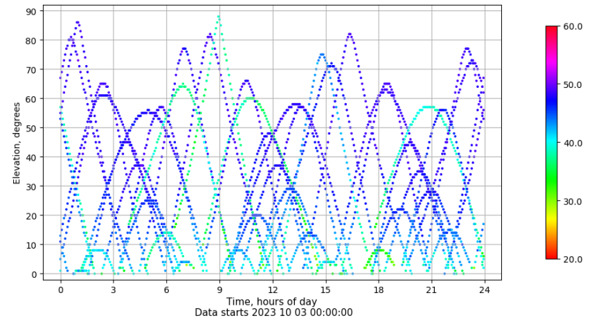
Time-elevation plot for station VALE. Signal to Noise S1C Data file VALE00ESP_R_2023276.xtr
