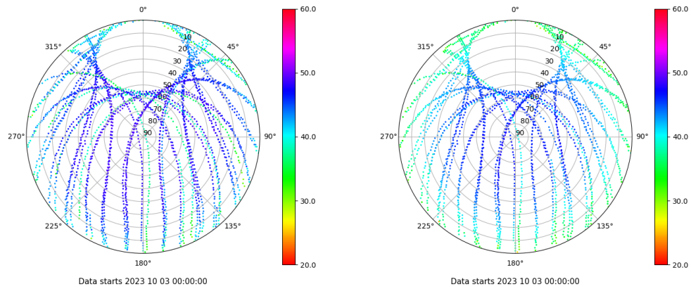
Skyplot for station VALE. Signal to Noise S1C Data file VALE00ESP_R_2023276.xtr Skyplot for station VALE. Signal to Noise S2P Data file VALE00ESP_R_2023276.xtr
