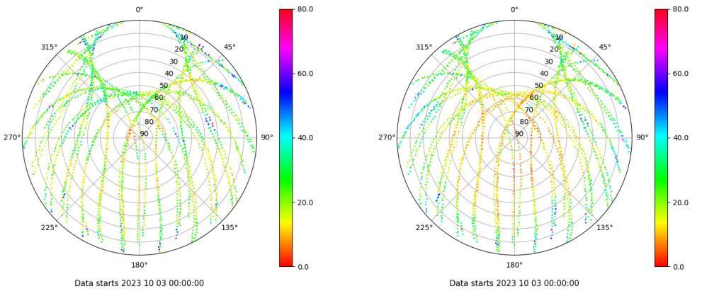
Skyplot for station VALE. Parameter M1C Data file VALE00ESP_R_2023276.xtr Skyplot for station VALE. Parameter M2P Data file VALE00ESP_R_2023276.xtr
