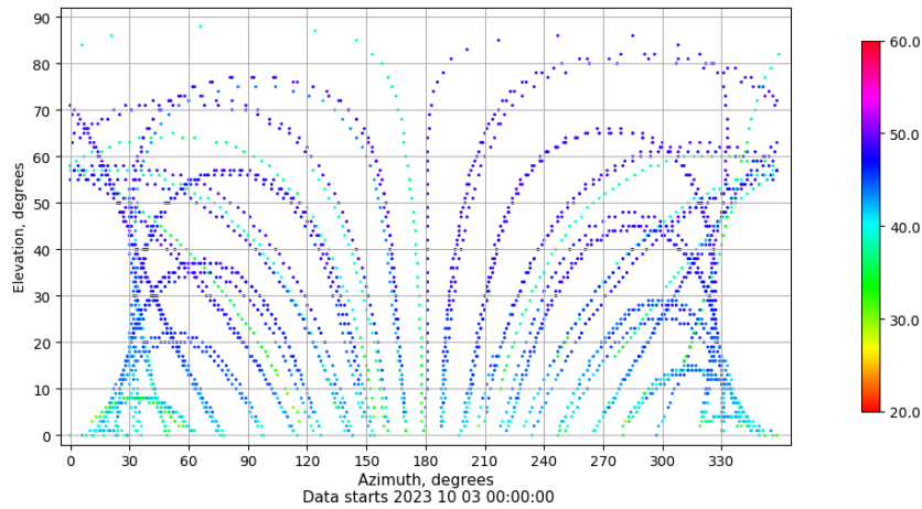
Azimuth-elevation plot for station VALE. Signal to Noise S1C Data file VALE00ESP_R_2023276.xtr
