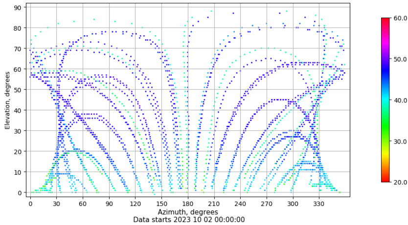
Azimuth-elevation plot for station VALE. Signal to Noise S1C Data file VALE00ESP_R_2023275.xtr
