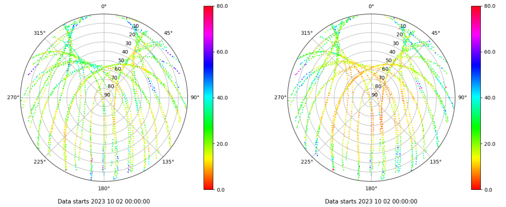
Skyplot for station VALE. Parameter M1C Data file VALE00ESP_R_2023275.xtr Skyplot for station VALE. Parameter M2P Data file VALE00ESP_R_2023275.xtr
