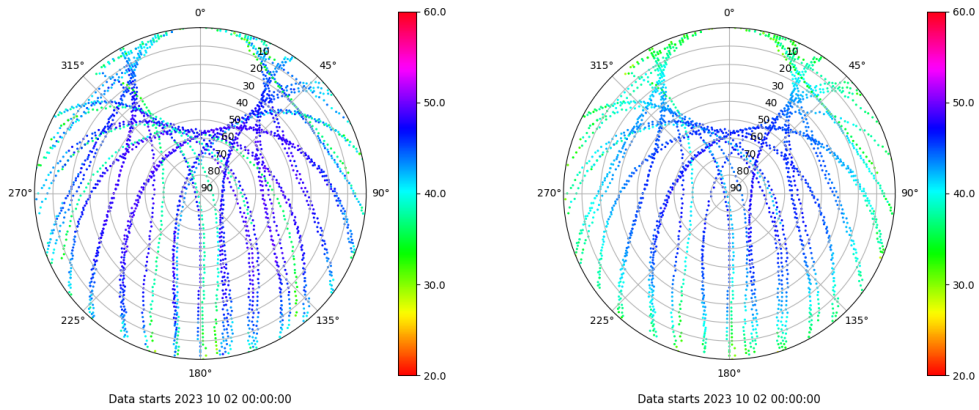
Skyplot for station VALE. Signal to Noise S1C Data file VALE00ESP_R_2023275.xtr Skyplot for station VALE. Signal to Noise S2P Data file VALE00ESP_R_2023275.xtr
