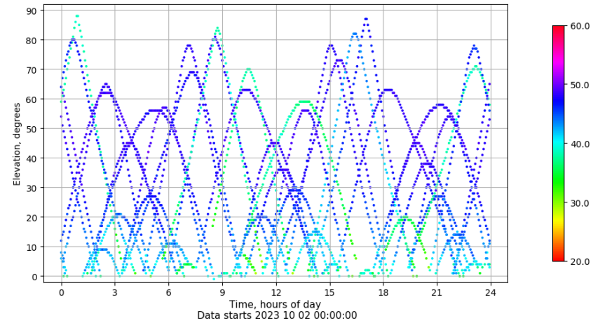
Time-elevation plot for station VALE. Signal to Noise S1C Data file VALE00ESP_R_2023275.xtr
