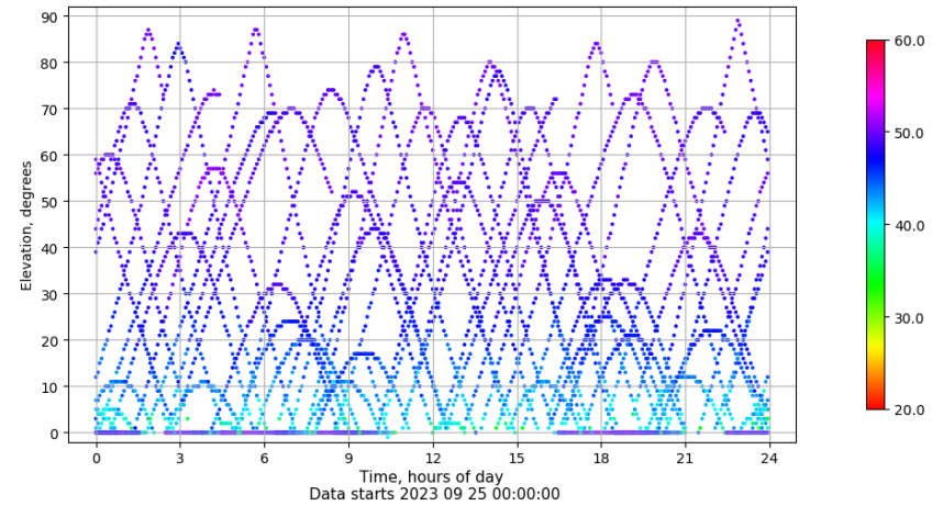
Time-elevation plot for station VALE. Signal to Noise S1C Data file VALE00ESP_R_2023268.xtr
