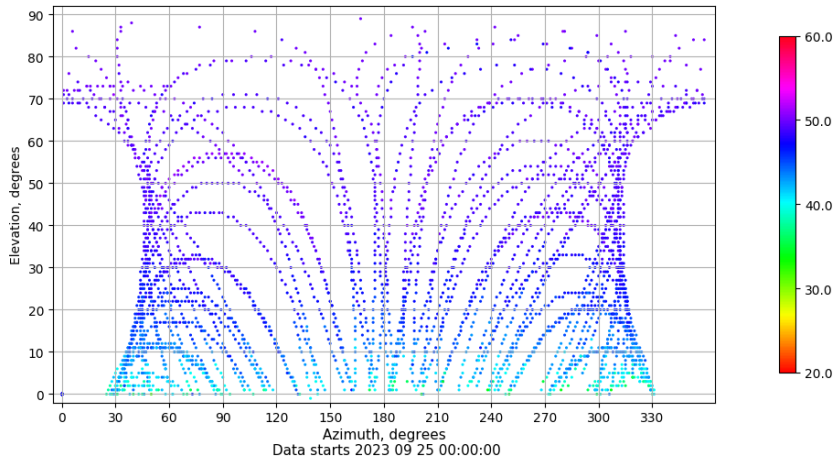
Azimuth-elevation plot for station VALE. Signal to Noise S1C Data file VALE00ESP_R_2023268.xtr
