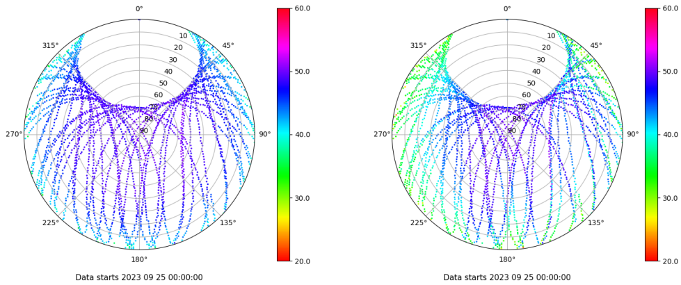
Skyplot for station VALE. Signal to Noise S1C Data file VALE00ESP_R_2023268.xtr Skyplot for station VALE. Signal to Noise S2W Data file VALE00ESP_R_2023268.xtr
