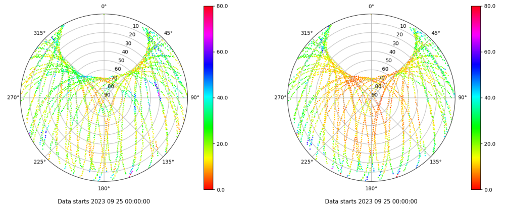
Skyplot for station VALE. Parameter M1C Data file VALE00ESP_R_2023268.xtr Skyplot for station VALE. Parameter M2W Data file VALE00ESP_R_2023268.xtr
