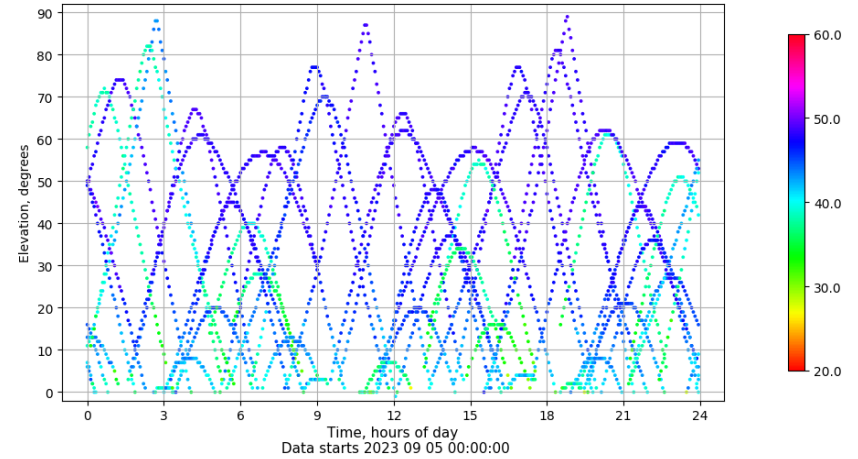
Time-elevation plot for station VALE. Signal to Noise S1C Data file VALE00ESP_R_2023248.xtr
