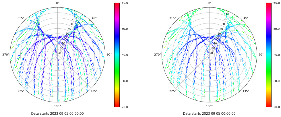
Skyplot for station VALE. Signal to Noise S1C Data file VALE00ESP_R_2023248.xtr Skyplot for station VALE. Signal to Noise S2P Data file VALE00ESP_R_2023248.xtr
