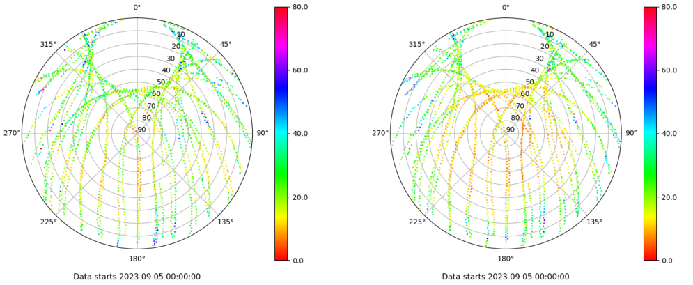
Skyplot for station VALE. Parameter M1C Data file VALE00ESP_R_2023248.xtr Skyplot for station VALE. Parameter M2P Data file VALE00ESP_R_2023248.xtr
