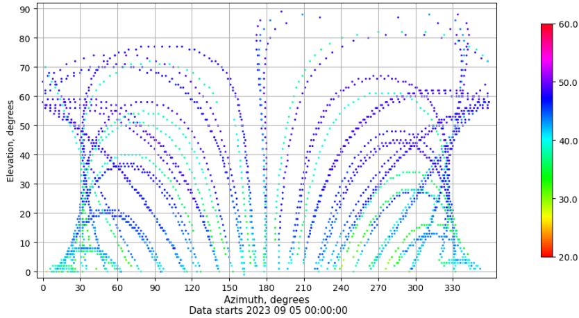
Azimuth-elevation plot for station VALE. Signal to Noise S1C Data file VALE00ESP_R_2023248.xtr
