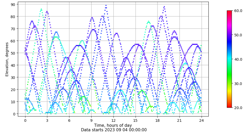
Time-elevation plot for station VALE. Signal to Noise S1C Data file VALE00ESP_R_2023247.xtr
