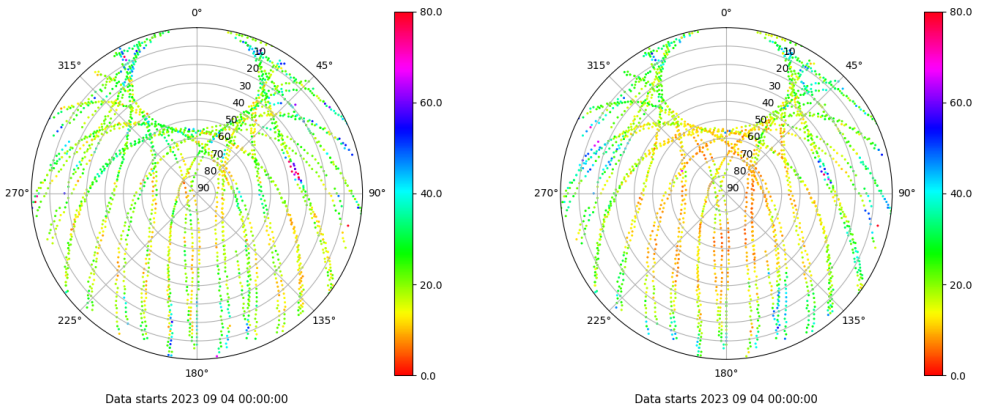
Skyplot for station VALE. Parameter M1C Data file VALE00ESP_R_2023247.xtr Skyplot for station VALE. Parameter M2P Data file VALE00ESP_R_2023247.xtr
