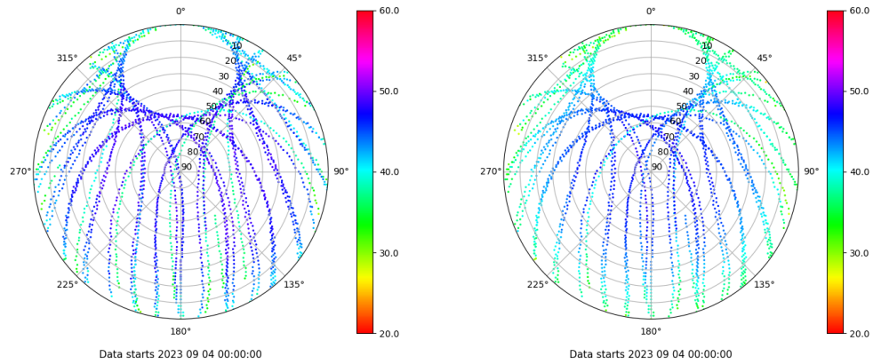
Skyplot for station VALE. Signal to Noise S1C Data file VALE00ESP_R_2023247.xtr Skyplot for station VALE. Signal to Noise S2P Data file VALE00ESP_R_2023247.xtr
