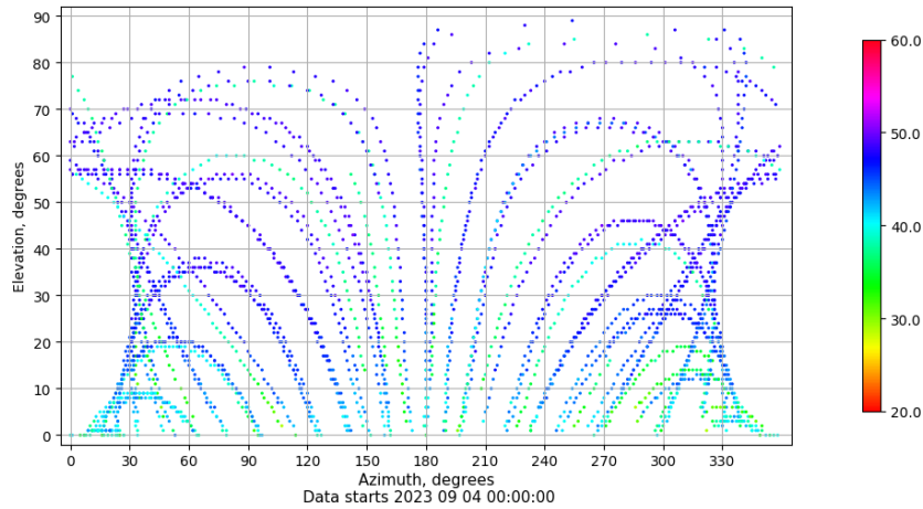
Azimuth-elevation plot for station VALE. Signal to Noise S1C Data file VALE00ESP_R_2023247.xtr
