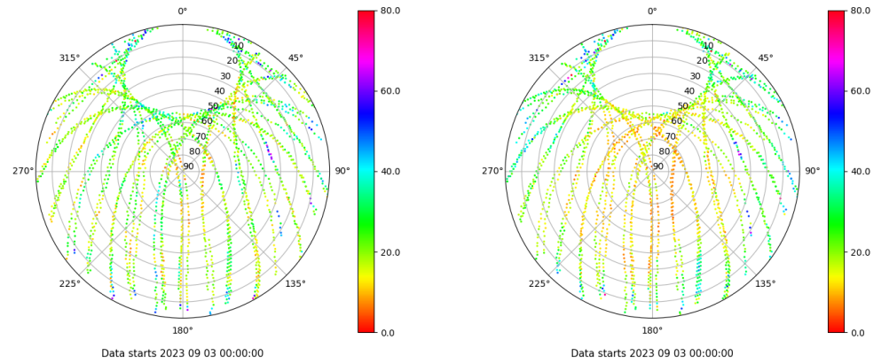
Skyplot for station VALE. Parameter M1C Data file VALE00ESP_R_2023246.xtr Skyplot for station VALE. Parameter M2P Data file VALE00ESP_R_2023246.xtr
