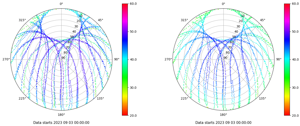
Skyplot for station VALE. Signal to Noise S1C Data file VALE00ESP_R_2023246.xtr Skyplot for station VALE. Signal to Noise S2P Data file VALE00ESP_R_2023246.xtr
