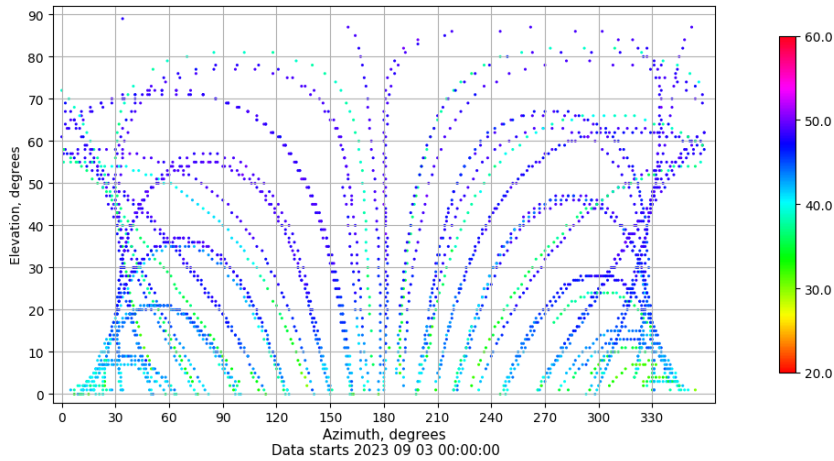
Azimuth-elevation plot for station VALE. Signal to Noise S1C Data file VALE00ESP_R_2023246.xtr
