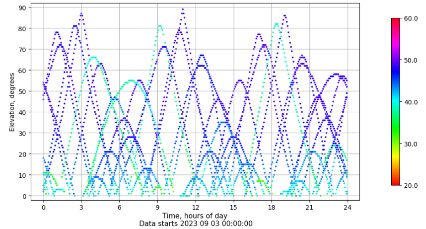
Time-elevation plot for station VALE. Signal to Noise S1C Data file VALE00ESP_R_2023246.xtr
