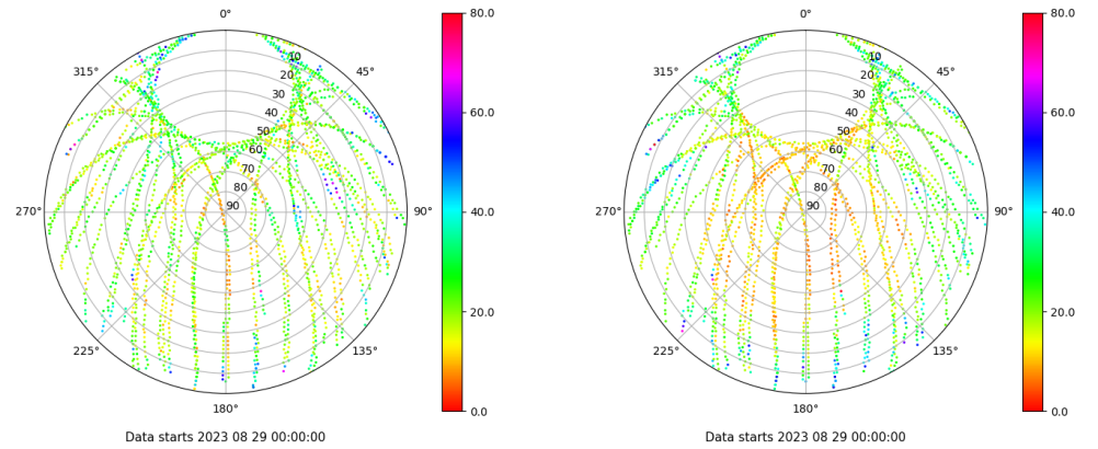
Skyplot for station VALE. Parameter M1C Data file VALE00ESP_R_2023241.xtr Skyplot for station VALE. Parameter M2P Data file VALE00ESP_R_2023241.xtr
