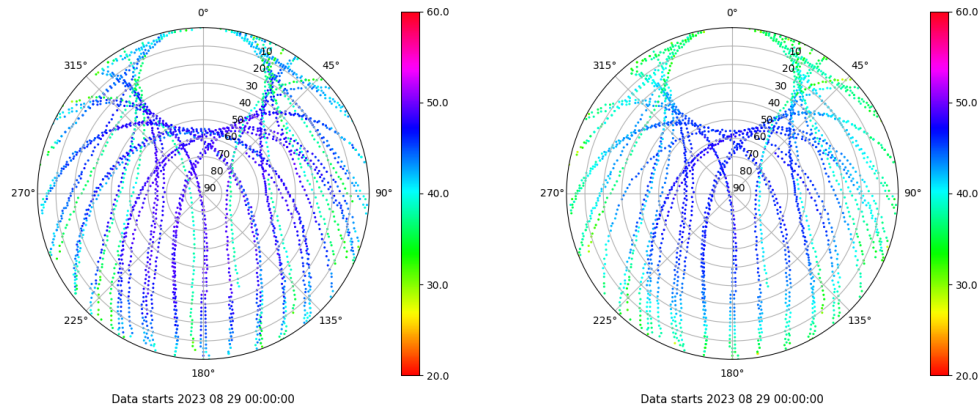
Skyplot for station VALE. Signal to Noise S1C Data file VALE00ESP_R_2023241.xtr Skyplot for station VALE. Signal to Noise S2P Data file VALE00ESP_R_2023241.xtr
