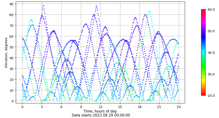
Time-elevation plot for station VALE. Signal to Noise S1C Data file VALE00ESP_R_2023241.xtr
