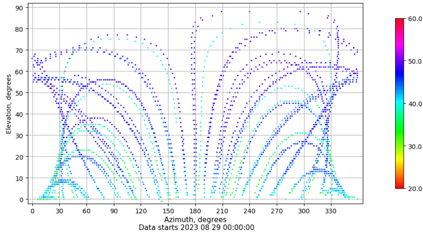
Azimuth-elevation plot for station VALE. Signal to Noise S1C Data file VALE00ESP_R_2023241.xtr
