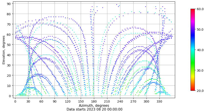
Azimuth-elevation plot for station VALE. Signal to Noise S1C Data file VALE00ESP_R_2023232.xtr
