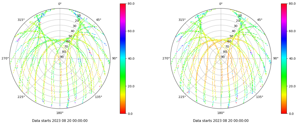
Skyplot for station VALE. Parameter M1C Data file VALE00ESP_R_2023232.xtr Skyplot for station VALE. Parameter M2P Data file VALE00ESP_R_2023232.xtr
