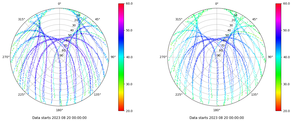
Skyplot for station VALE. Signal to Noise S1C Data file VALE00ESP_R_2023232.xtr Skyplot for station VALE. Signal to Noise S2P Data file VALE00ESP_R_2023232.xtr
