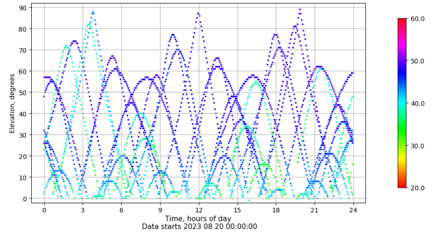
Time-elevation plot for station VALE. Signal to Noise S1C Data file VALE00ESP_R_2023232.xtr
