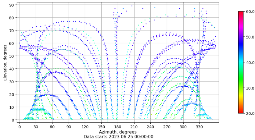
Azimuth-elevation plot for station VALE. Signal to Noise S1C Data file VALE00ESP_R_2023176.xtr
