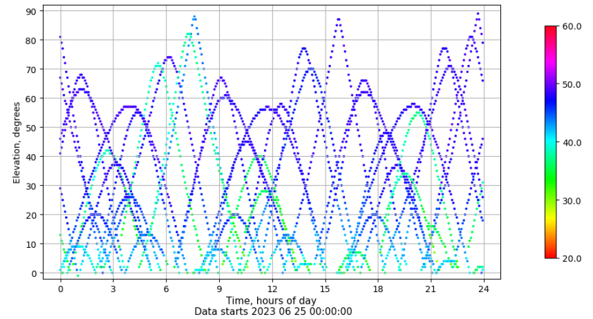
Time-elevation plot for station VALE. Signal to Noise S1C Data file VALE00ESP_R_2023176.xtr
