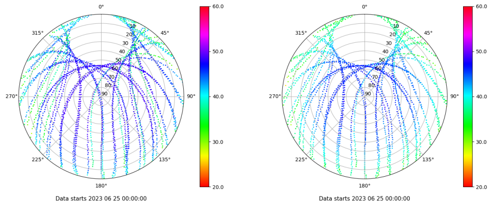
Skyplot for station VALE. Signal to Noise S1C Data file VALE00ESP_R_2023176.xtr Skyplot for station VALE. Signal to Noise S2P Data file VALE00ESP_R_2023176.xtr
