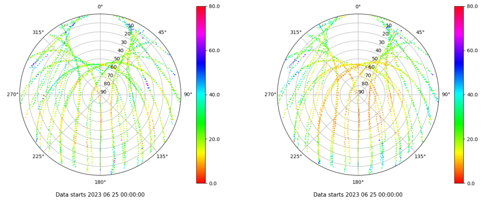
Skyplot for station VALE. Parameter M1C Data file VALE00ESP_R_2023176.xtr Skyplot for station VALE. Parameter M2P Data file VALE00ESP_R_2023176.xtr
