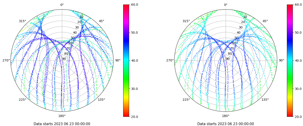
Skyplot for station VALE. Signal to Noise S1C Data file VALE00ESP_R_2023174.xtr Skyplot for station VALE. Signal to Noise S2P Data file VALE00ESP_R_2023174.xtr
