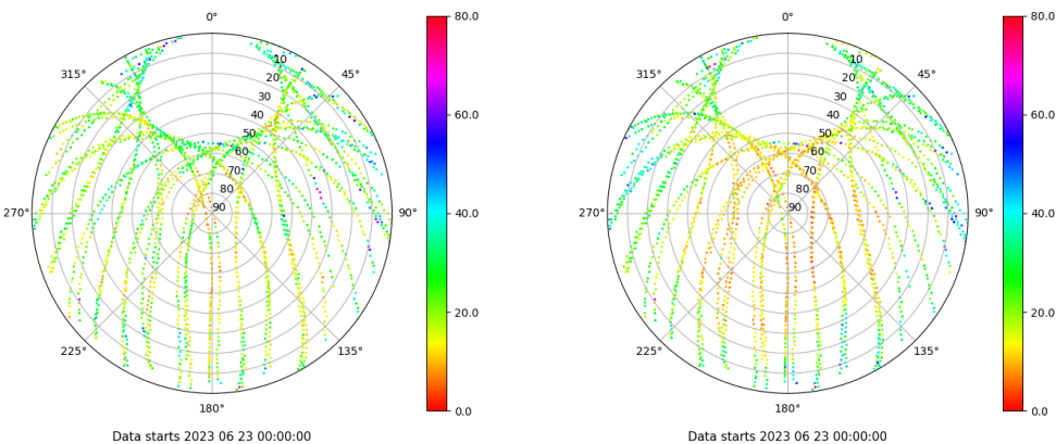
Skyplot for station VALE. Parameter M1C Data file VALE00ESP_R_2023174.xtr Skyplot for station VALE. Parameter M2P Data file VALE00ESP_R_2023174.xtr
