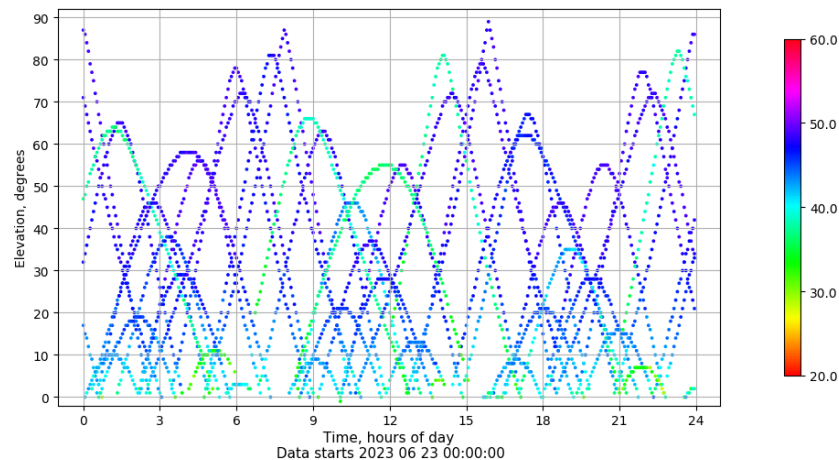
Time-elevation plot for station VALE. Signal to Noise S1C Data file VALE00ESP_R_2023174.xtr
