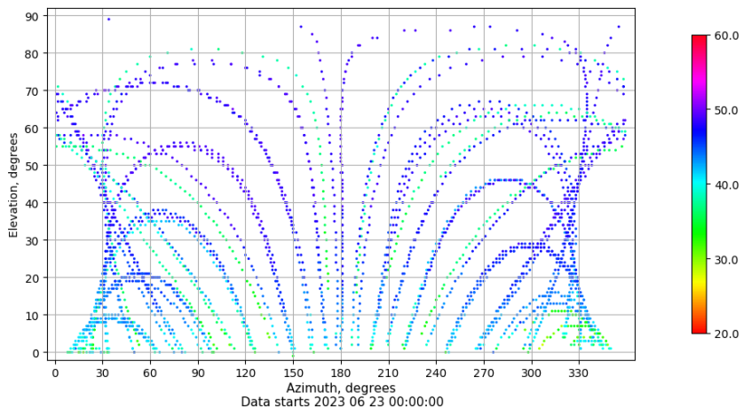
Azimuth-elevation plot for station VALE. Signal to Noise S1C Data file VALE00ESP_R_2023174.xtr
