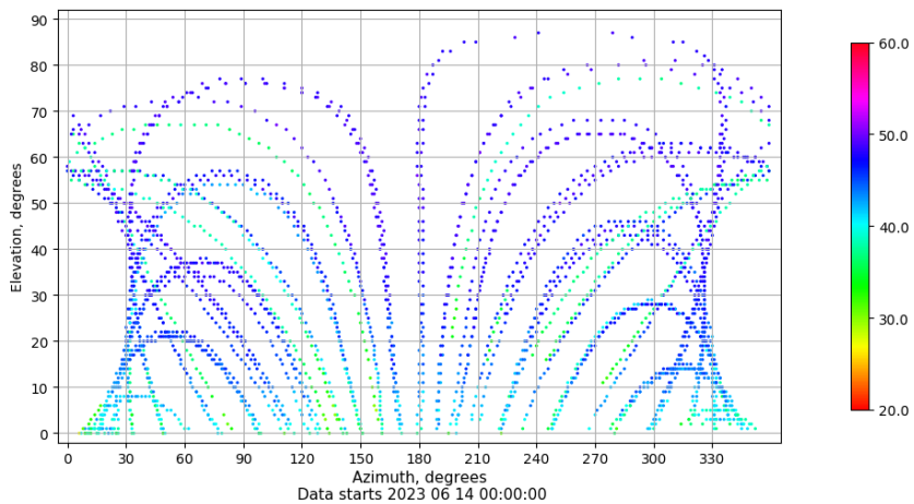
Azimuth-elevation plot for station VALE. Signal to Noise S1C Data file VALE00ESP_R_2023165.xtr
