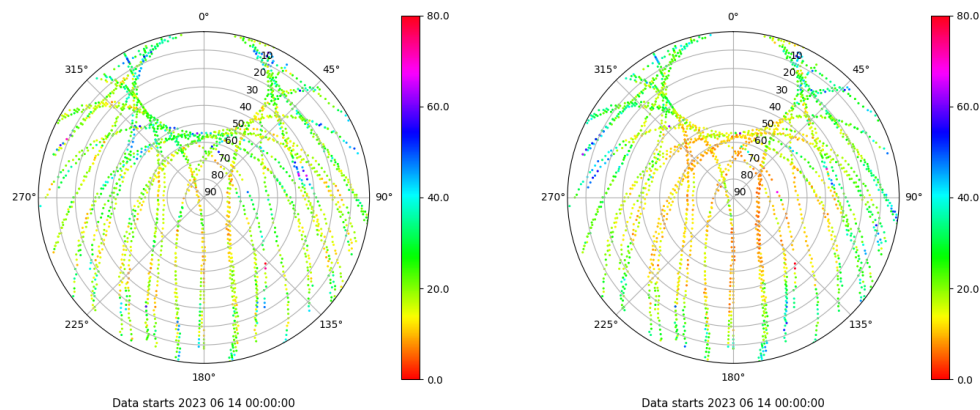
Skyplot for station VALE. Parameter M1C Data file VALE00ESP_R_2023165.xtr Skyplot for station VALE. Parameter M2P Data file VALE00ESP_R_2023165.xtr
