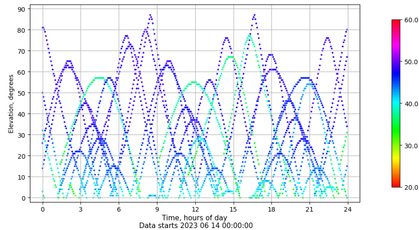
Time-elevation plot for station VALE. Signal to Noise S1C Data file VALE00ESP_R_2023165.xtr
