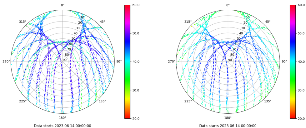
Skyplot for station VALE. Signal to Noise S1C Data file VALE00ESP_R_2023165.xtr Skyplot for station VALE. Signal to Noise S2P Data file VALE00ESP_R_2023165.xtr
