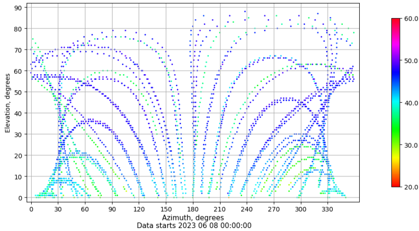
Azimuth-elevation plot for station VALE. Signal to Noise S1C Data file VALE00ESP_R_2023159.xtr
