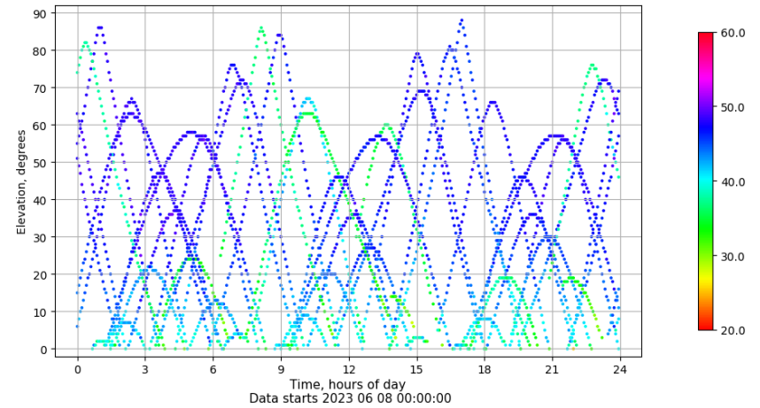
Time-elevation plot for station VALE. Signal to Noise S1C Data file VALE00ESP_R_2023159.xtr
