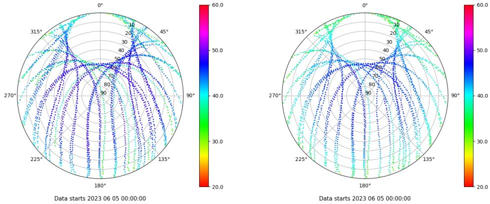
Skyplot for station VALE. Signal to Noise S1C Data file VALE00ESP_R_2023156.xtr Skyplot for station VALE. Signal to Noise S2P Data file VALE00ESP_R_2023156.xtr
