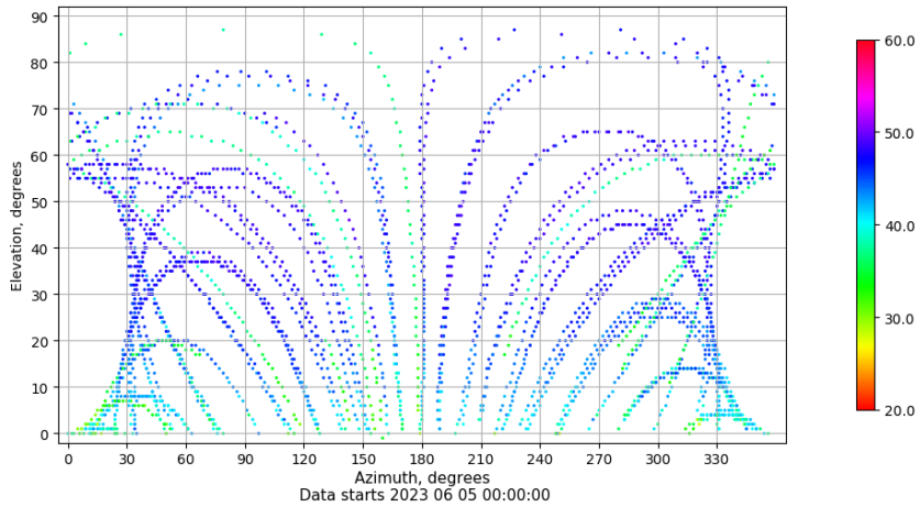
Azimuth-elevation plot for station VALE. Signal to Noise S1C Data file VALE00ESP_R_2023156.xtr
