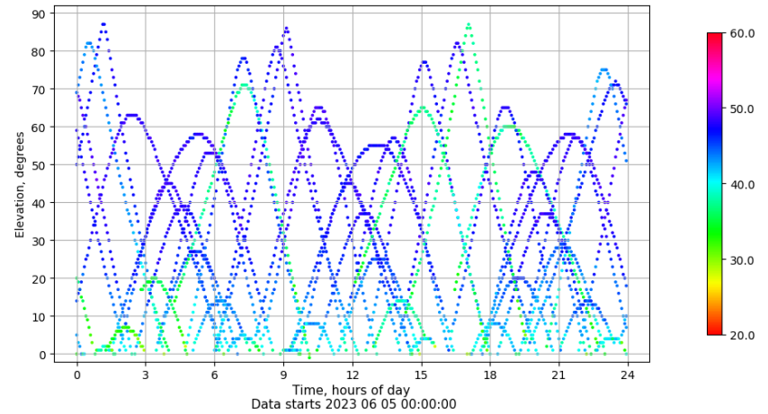
Time-elevation plot for station VALE. Signal to Noise S1C Data file VALE00ESP_R_2023156.xtr
