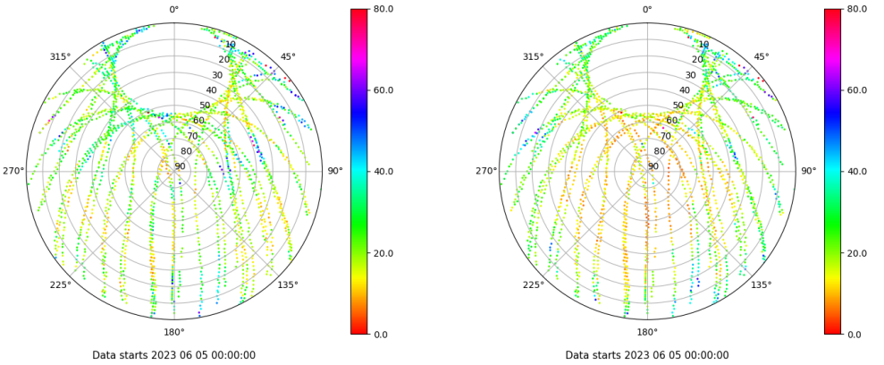
Skyplot for station VALE. Parameter M1C Data file VALE00ESP_R_2023156.xtr Skyplot for station VALE. Parameter M2P Data file VALE00ESP_R_2023156.xtr
