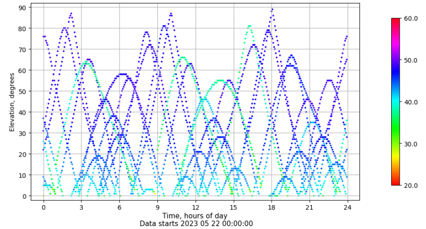
Time-elevation plot for station VALE. Signal to Noise S1C Data file VALE00ESP_R_2023142.xtr
