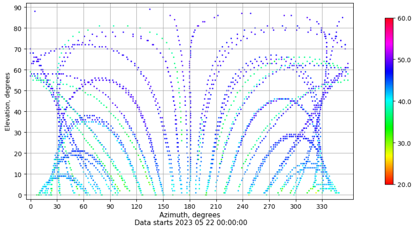
Azimuth-elevation plot for station VALE. Signal to Noise S1C Data file VALE00ESP_R_2023142.xtr
