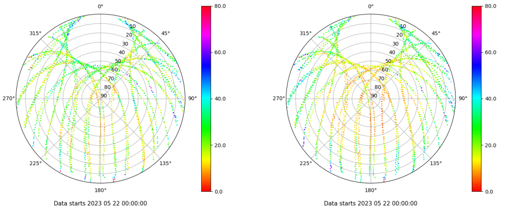
Skyplot for station VALE. Parameter M1C Data file VALE00ESP_R_2023142.xtr Skyplot for station VALE. Parameter M2P Data file VALE00ESP_R_2023142.xtr
