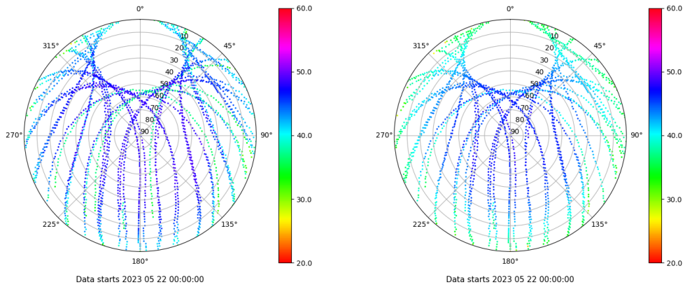
Skyplot for station VALE. Signal to Noise S1C Data file VALE00ESP_R_2023142.xtr Skyplot for station VALE. Signal to Noise S2P Data file VALE00ESP_R_2023142.xtr
