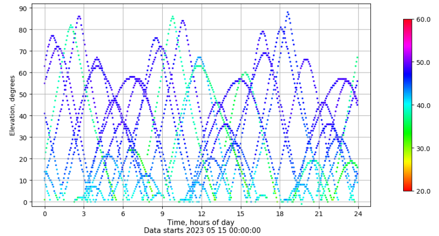
Time-elevation plot for station VALE. Signal to Noise S1C Data file VALE00ESP_R_2023135.xtr
