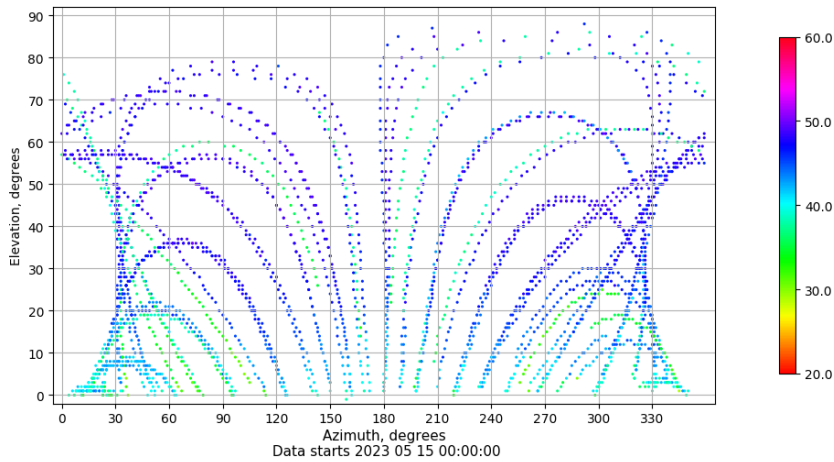
Azimuth-elevation plot for station VALE. Signal to Noise S1C Data file VALE00ESP_R_2023135.xtr
