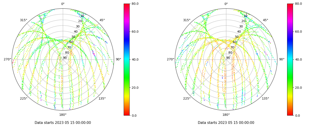
Skyplot for station VALE. Parameter M1C Data file VALE00ESP_R_2023135.xtr Skyplot for station VALE. Parameter M2P Data file VALE00ESP_R_2023135.xtr
