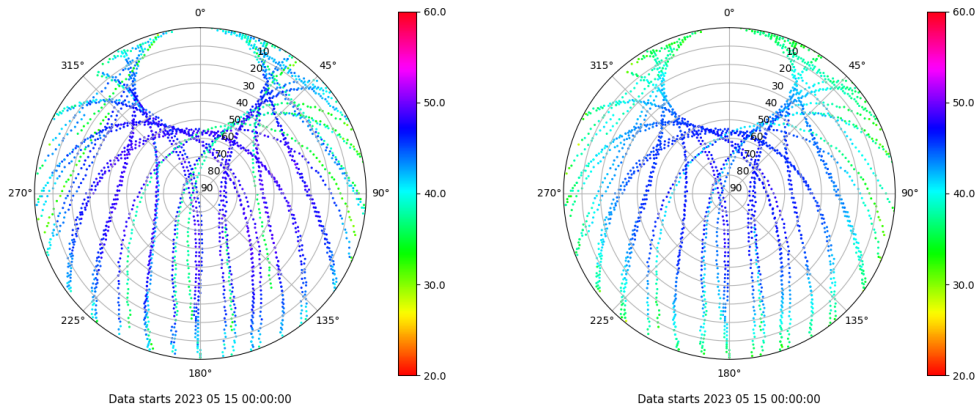
Skyplot for station VALE. Signal to Noise S1C Data file VALE00ESP_R_2023135.xtr Skyplot for station VALE. Signal to Noise S2P Data file VALE00ESP_R_2023135.xtr
