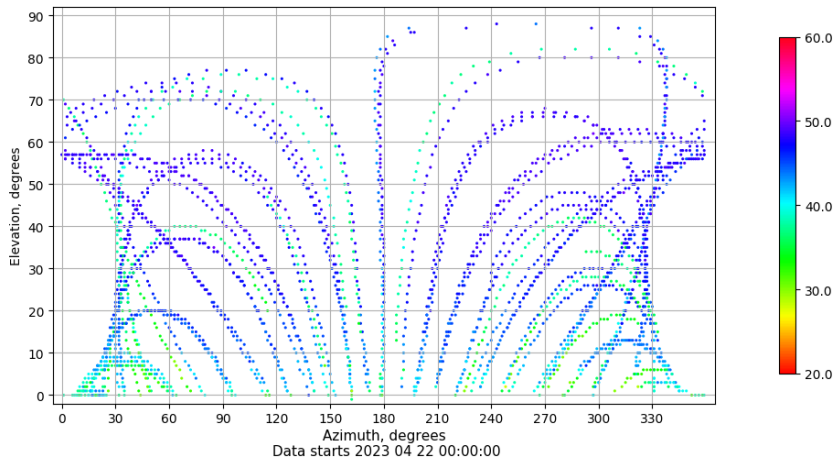
Azimuth-elevation plot for station VALE. Signal to Noise S1C Data file VALE00ESP_R_2023112.xtr
