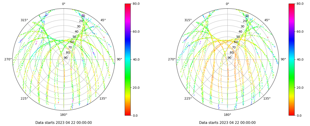
Skyplot for station VALE. Parameter M1C Data file VALE00ESP_R_2023112.xtr Skyplot for station VALE. Parameter M2P Data file VALE00ESP_R_2023112.xtr
