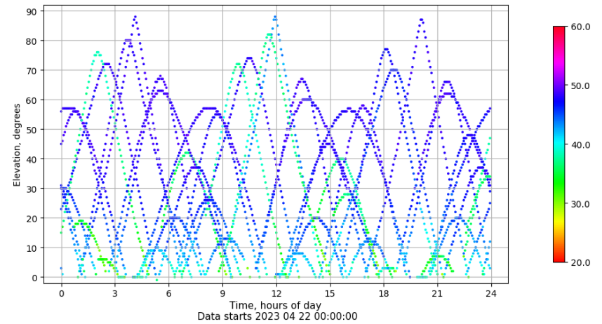
Time-elevation plot for station VALE. Signal to Noise S1C Data file VALE00ESP_R_2023112.xtr
