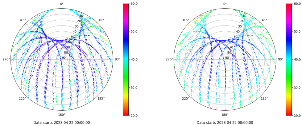
Skyplot for station VALE. Signal to Noise S1C Data file VALE00ESP_R_2023112.xtr Skyplot for station VALE. Signal to Noise S2P Data file VALE00ESP_R_2023112.xtr
