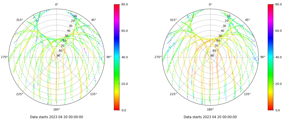
Skyplot for station VALE. Parameter M1C Data file VALE00ESP_R_2023110.xtr Skyplot for station VALE. Parameter M2P Data file VALE00ESP_R_2023110.xtr
