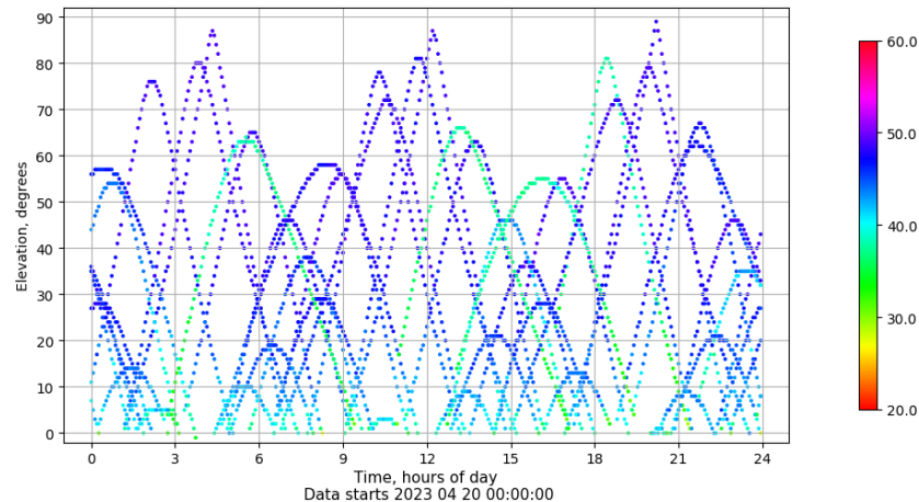
Time-elevation plot for station VALE. Signal to Noise S1C Data file VALE00ESP_R_2023110.xtr
