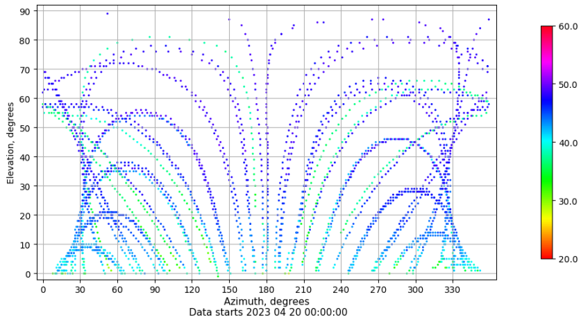
Azimuth-elevation plot for station VALE. Signal to Noise S1C Data file VALE00ESP_R_2023110.xtr
