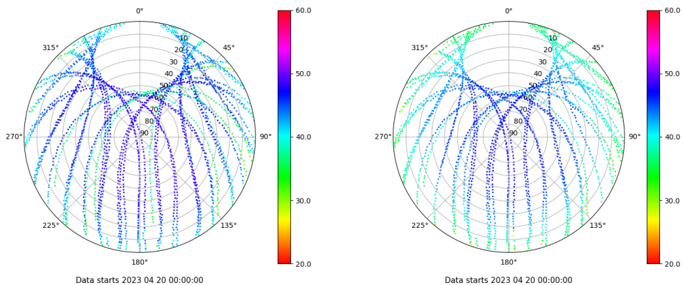
Skyplot for station VALE. Signal to Noise S1C Data file VALE00ESP_R_2023110.xtr Skyplot for station VALE. Signal to Noise S2P Data file VALE00ESP_R_2023110.xtr
