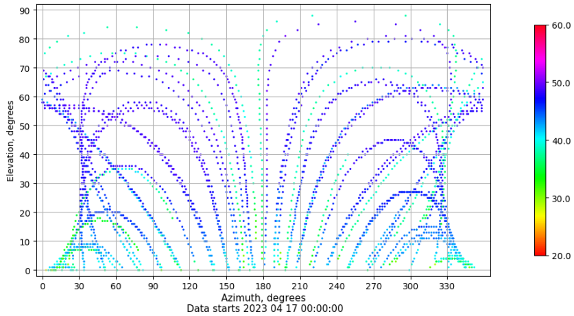
Azimuth-elevation plot for station VALE. Signal to Noise S1C Data file VALE00ESP_R_2023107.xtr
