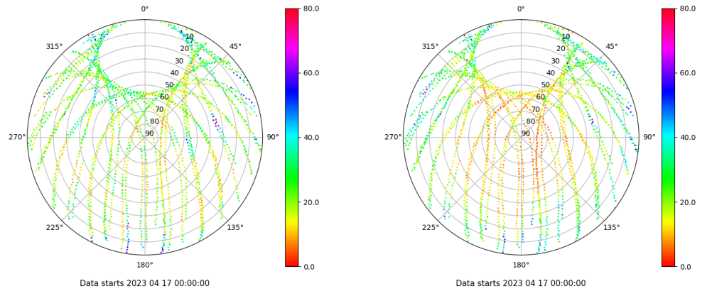
Skyplot for station VALE. Parameter M1C Data file VALE00ESP_R_2023107.xtr Skyplot for station VALE. Parameter M2P Data file VALE00ESP_R_2023107.xtr
