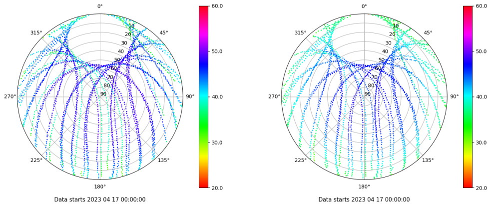
Skyplot for station VALE. Signal to Noise S1C Data file VALE00ESP_R_2023107.xtr Skyplot for station VALE. Signal to Noise S2P Data file VALE00ESP_R_2023107.xtr
