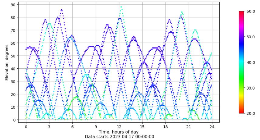
Time-elevation plot for station VALE. Signal to Noise S1C Data file VALE00ESP_R_2023107.xtr
