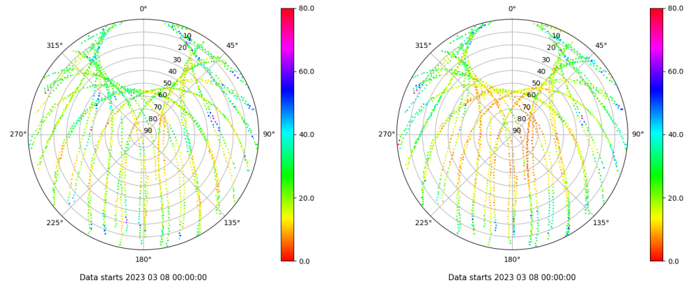
Skyplot for station VALE. Parameter M1C Data file VALE00ESP_R_2023067.xtr Skyplot for station VALE. Parameter M2P Data file VALE00ESP_R_2023067.xtr
