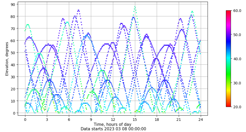
Time-elevation plot for station VALE. Signal to Noise S1C Data file VALE00ESP_R_2023067.xtr
