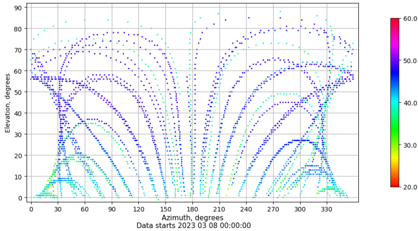
Azimuth-elevation plot for station VALE. Signal to Noise S1C Data file VALE00ESP_R_2023067.xtr
