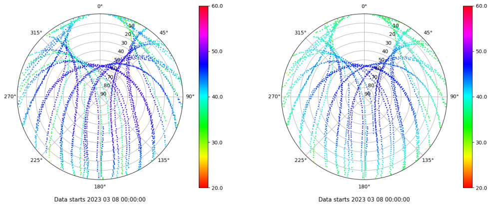
Skyplot for station VALE. Signal to Noise S1C Data file VALE00ESP_R_2023067.xtr Skyplot for station VALE. Signal to Noise S2P Data file VALE00ESP_R_2023067.xtr
