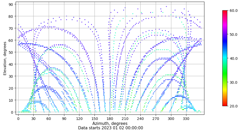
Azimuth-elevation plot for station VALE. Signal to Noise S1C Data file VALE00ESP_R_2023002.xtr
