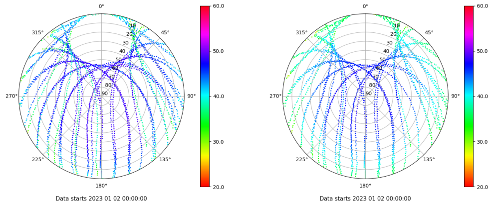
Skyplot for station VALE. Signal to Noise S1C Data file VALE00ESP_R_2023002.xtr Skyplot for station VALE. Signal to Noise S2P Data file VALE00ESP_R_2023002.xtr
