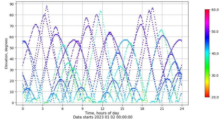
Time-elevation plot for station VALE. Signal to Noise S1C Data file VALE00ESP_R_2023002.xtr
