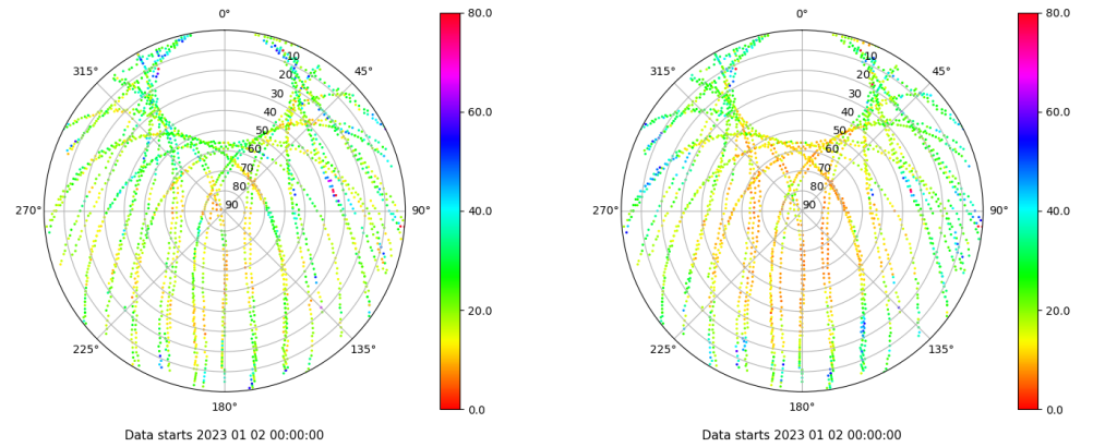
Skyplot for station VALE. Parameter M1C Data file VALE00ESP_R_2023002.xtr Skyplot for station VALE. Parameter M2P Data file VALE00ESP_R_2023002.xtr
