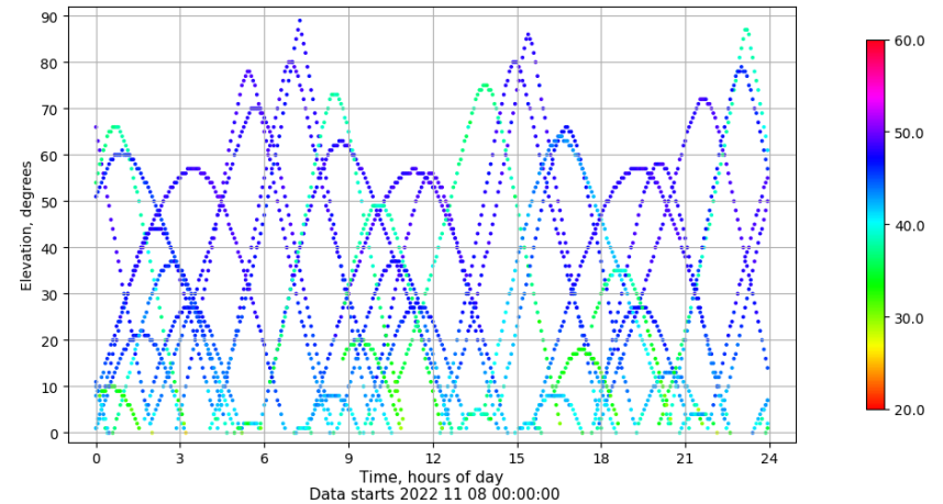
Time-elevation plot for station VALE. Signal to Noise S1C Data file VALE00ESP_R_2022312.xtr
