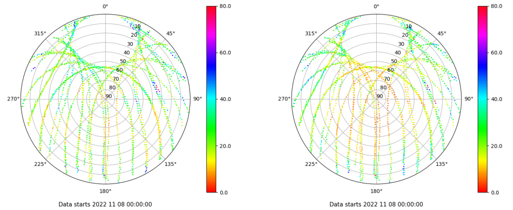
Skyplot for station VALE. Parameter M1C Data file VALE00ESP_R_2022312.xtr Skyplot for station VALE. Parameter M2P Data file VALE00ESP_R_2022312.xtr
