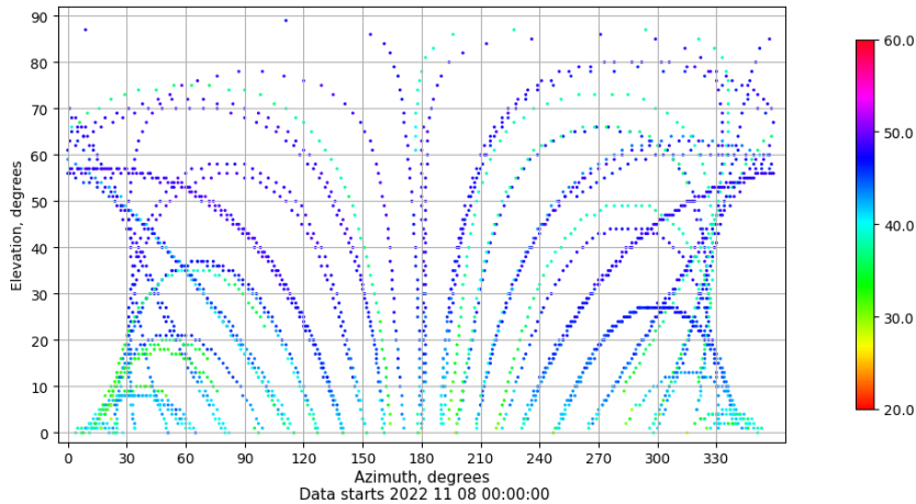
Azimuth-elevation plot for station VALE. Signal to Noise S1C Data file VALE00ESP_R_2022312.xtr
