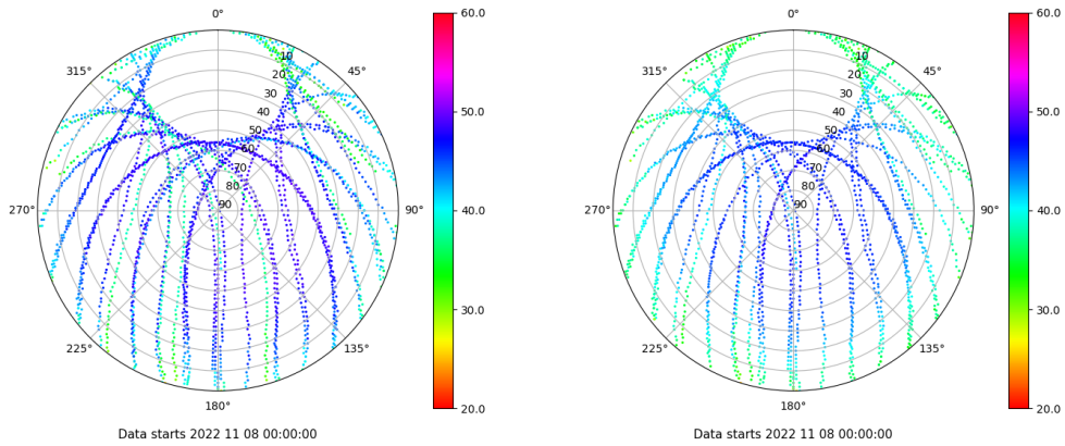
Skyplot for station VALE. Signal to Noise S1C Data file VALE00ESP_R_2022312.xtr Skyplot for station VALE. Signal to Noise S2P Data file VALE00ESP_R_2022312.xtr
