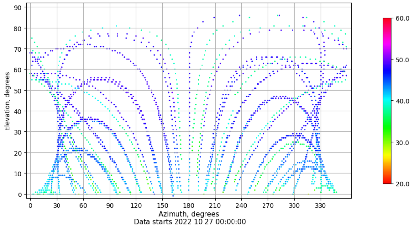
Azimuth-elevation plot for station VALE. Signal to Noise S1C Data file VALE00ESP_R_2022300.xtr
