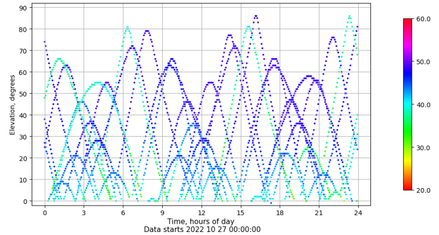
Time-elevation plot for station VALE. Signal to Noise S1C Data file VALE00ESP_R_2022300.xtr
