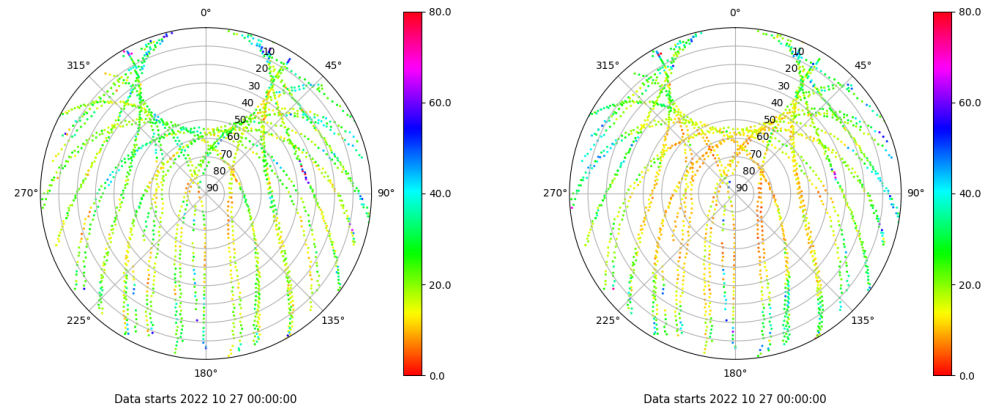
Skyplot for station VALE. Parameter M1C Data file VALE00ESP_R_2022300.xtr Skyplot for station VALE. Parameter M2P Data file VALE00ESP_R_2022300.xtr
