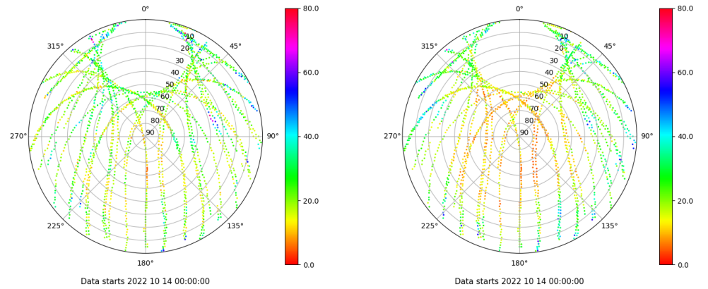
Skyplot for station VALE. Parameter M1C Data file VALE00ESP_R_2022287.xtr Skyplot for station VALE. Parameter M2P Data file VALE00ESP_R_2022287.xtr
