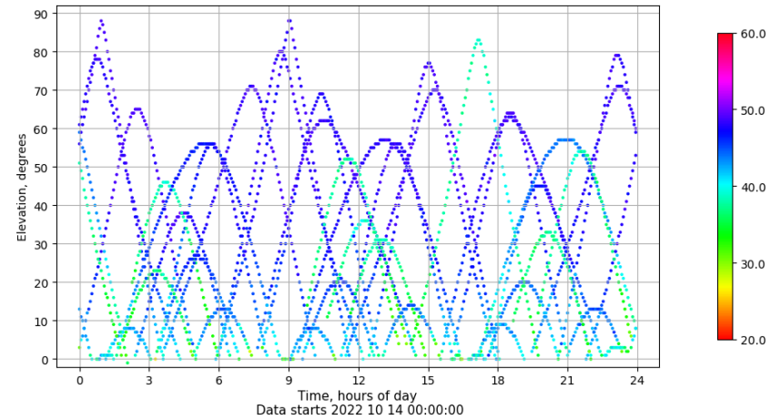
Time-elevation plot for station VALE. Signal to Noise S1C Data file VALE00ESP_R_2022287.xtr
