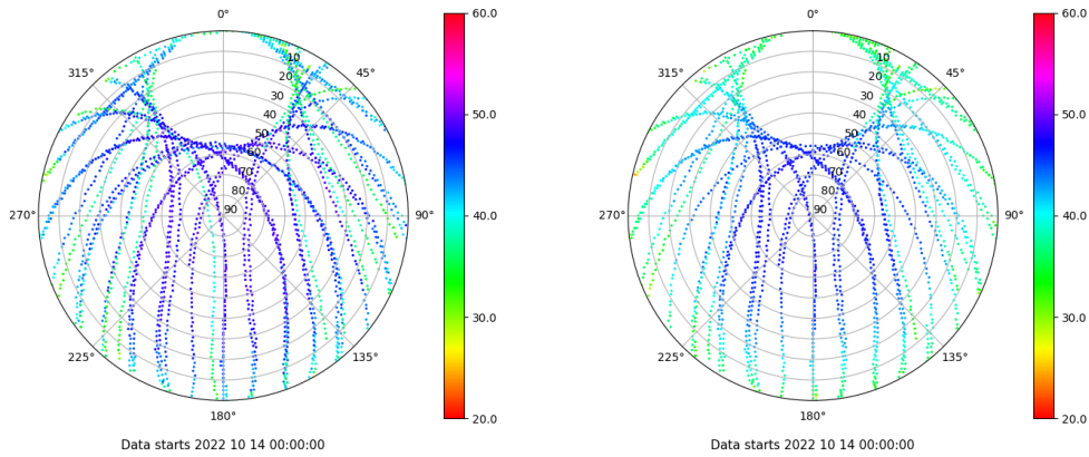
Skyplot for station VALE. Signal to Noise S1C Data file VALE00ESP_R_2022287.xtr Skyplot for station VALE. Signal to Noise S2P Data file VALE00ESP_R_2022287.xtr
