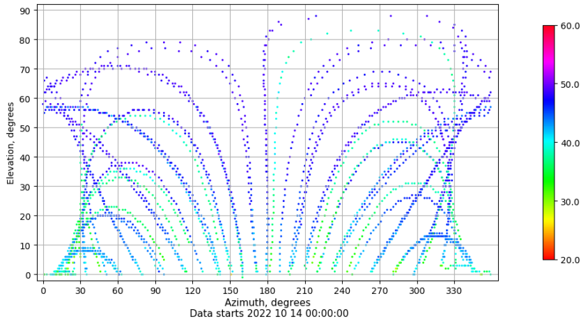
Azimuth-elevation plot for station VALE. Signal to Noise S1C Data file VALE00ESP_R_2022287.xtr
