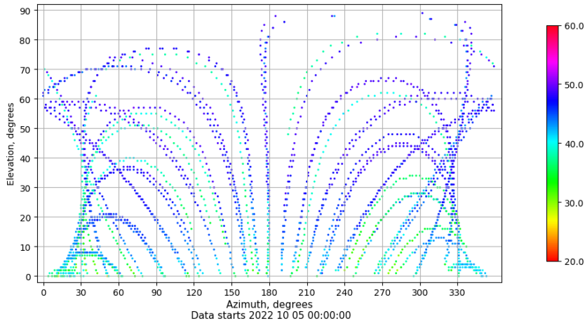
Azimuth-elevation plot for station VALE. Signal to Noise S1C Data file VALE00ESP_R_2022278.xtr
