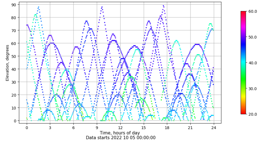
Time-elevation plot for station VALE. Signal to Noise S1C Data file VALE00ESP_R_2022278.xtr
