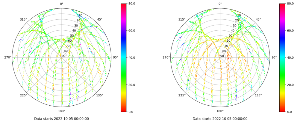
Skyplot for station VALE. Parameter M1C Data file VALE00ESP_R_2022278.xtr Skyplot for station VALE. Parameter M2P Data file VALE00ESP_R_2022278.xtr
