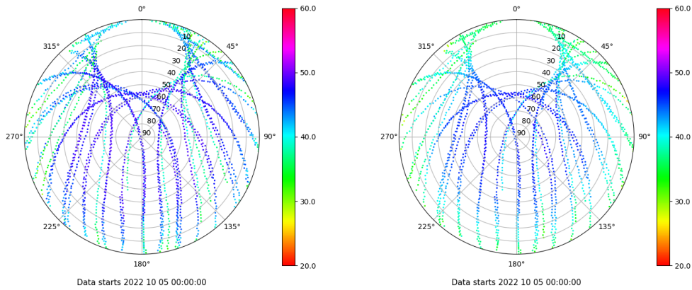
Skyplot for station VALE. Signal to Noise S1C Data file VALE00ESP_R_2022278.xtr Skyplot for station VALE. Signal to Noise S2P Data file VALE00ESP_R_2022278.xtr
