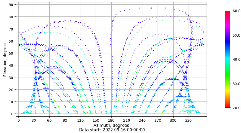
Azimuth-elevation plot for station VALE. Signal to Noise S1C Data file VALE00ESP_R_2022259.xtr
