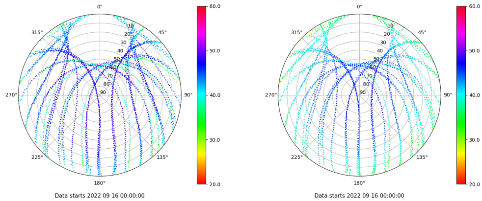
Skyplot for station VALE. Signal to Noise S1C Data file VALE00ESP_R_2022259.xtr Skyplot for station VALE. Signal to Noise S2P Data file VALE00ESP_R_2022259.xtr
