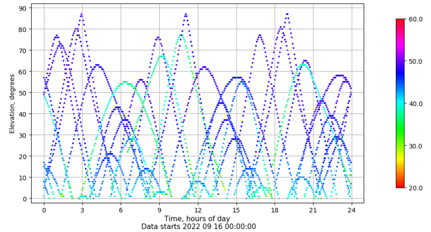
Time-elevation plot for station VALE. Signal to Noise S1C Data file VALE00ESP_R_2022259.xtr
