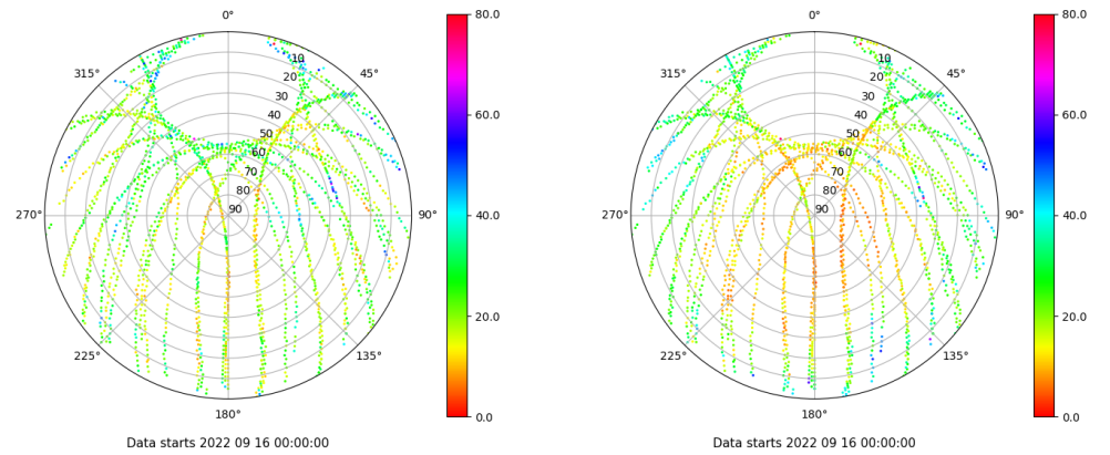
Skyplot for station VALE. Parameter M1C Data file VALE00ESP_R_2022259.xtr Skyplot for station VALE. Parameter M2P Data file VALE00ESP_R_2022259.xtr
