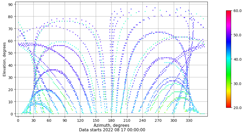
Azimuth-elevation plot for station VALE. Signal to Noise S1C Data file VALE00ESP_R_2022229.xtr
