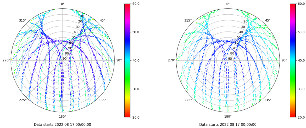
Skyplot for station VALE. Signal to Noise S1C Data file VALE00ESP_R_2022229.xtr Skyplot for station VALE. Signal to Noise S2P Data file VALE00ESP_R_2022229.xtr
