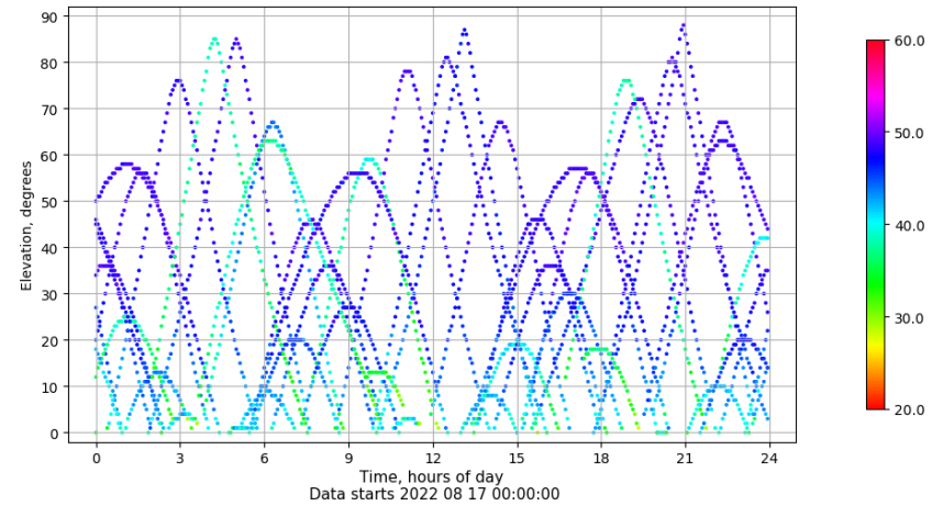
Time-elevation plot for station VALE. Signal to Noise S1C Data file VALE00ESP_R_2022229.xtr
