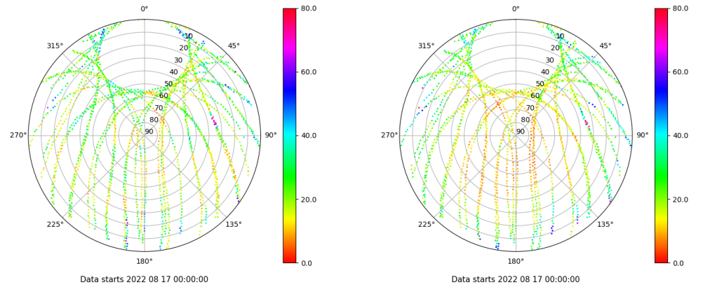
Skyplot for station VALE. Parameter M1C Data file VALE00ESP_R_2022229.xtr Skyplot for station VALE. Parameter M2P Data file VALE00ESP_R_2022229.xtr
