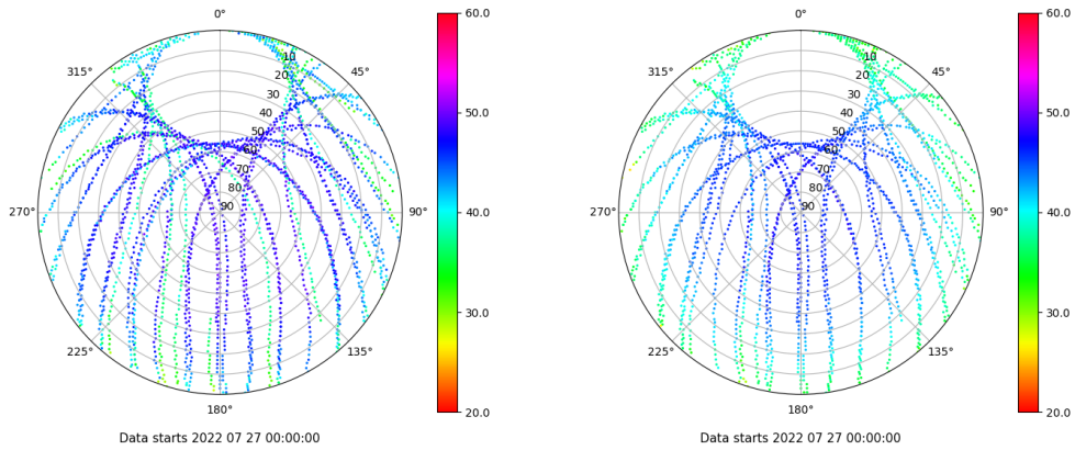
Skyplot for station VALE. Signal to Noise S1C Data file VALE00ESP_R_2022208.xtr Skyplot for station VALE. Signal to Noise S2P Data file VALE00ESP_R_2022208.xtr
