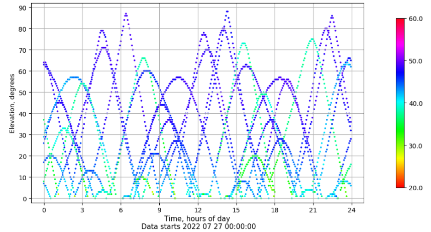
Time-elevation plot for station VALE. Signal to Noise S1C Data file VALE00ESP_R_2022208.xtr
