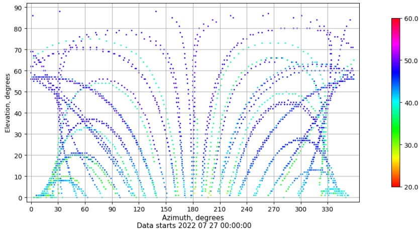
Azimuth-elevation plot for station VALE. Signal to Noise S1C Data file VALE00ESP_R_2022208.xtr
