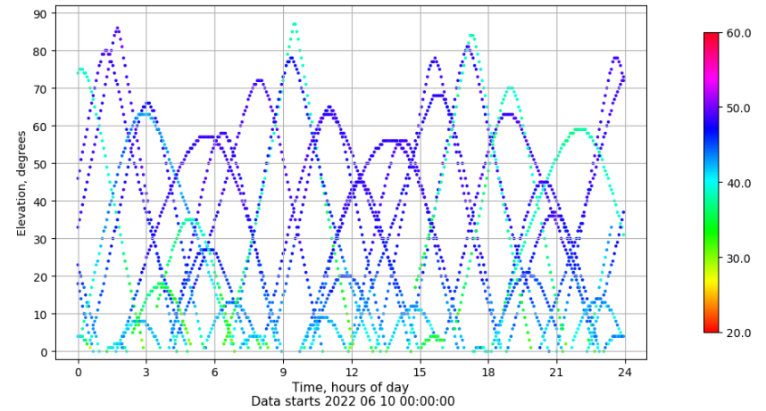
Time-elevation plot for station VALE. Signal to Noise S1C Data file VALE00ESP_R_2022161.xtr
