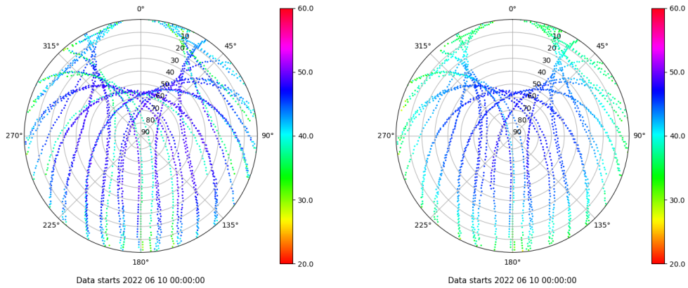
Skyplot for station VALE. Signal to Noise S1C Data file VALE00ESP_R_2022161.xtr Skyplot for station VALE. Signal to Noise S2P Data file VALE00ESP_R_2022161.xtr
