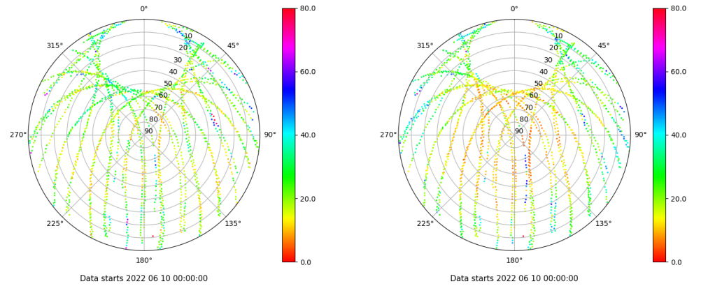
Skyplot for station VALE. Parameter M1C Data file VALE00ESP_R_2022161.xtr Skyplot for station VALE. Parameter M2P Data file VALE00ESP_R_2022161.xtr
