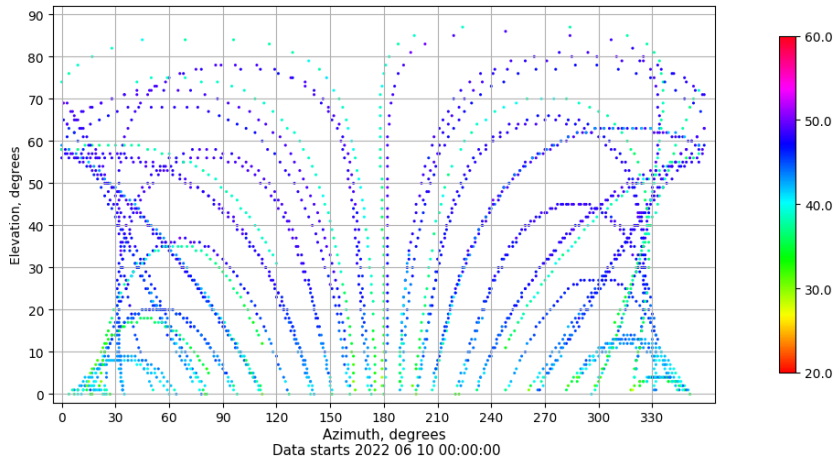
Azimuth-elevation plot for station VALE. Signal to Noise S1C Data file VALE00ESP_R_2022161.xtr
