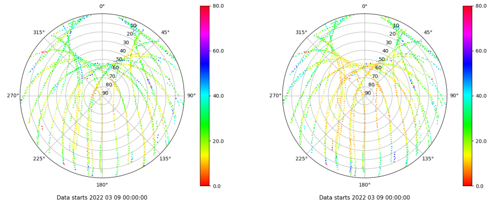
Skyplot for station VALE. Parameter M1C Data file VALE00ESP_R_2022068.xtr Skyplot for station VALE. Parameter M2P Data file VALE00ESP_R_2022068.xtr
