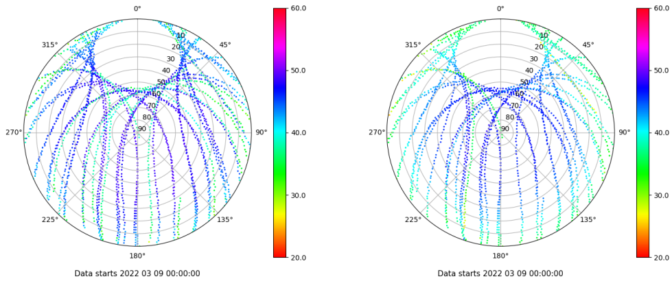
Skyplot for station VALE. Signal to Noise S1C Data file VALE00ESP_R_2022068.xtr Skyplot for station VALE. Signal to Noise S2P Data file VALE00ESP_R_2022068.xtr
