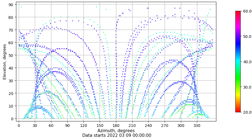
Azimuth-elevation plot for station VALE. Signal to Noise S1C Data file VALE00ESP_R_2022068.xtr
