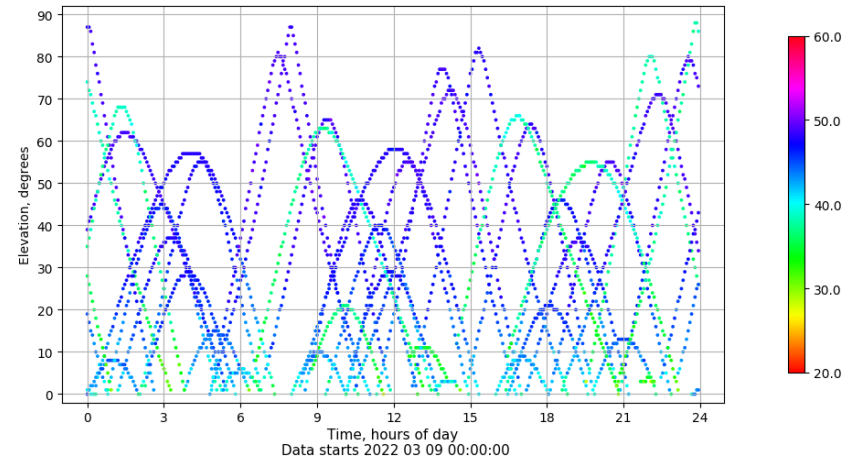
Time-elevation plot for station VALE. Signal to Noise S1C Data file VALE00ESP_R_2022068.xtr
