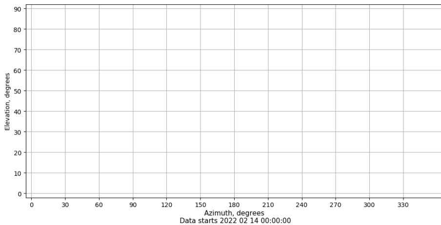
Azimuth-elevation plot for station VALE. Signal to Noise S1C Data file VALE00ESP_R_2022045.xtr
