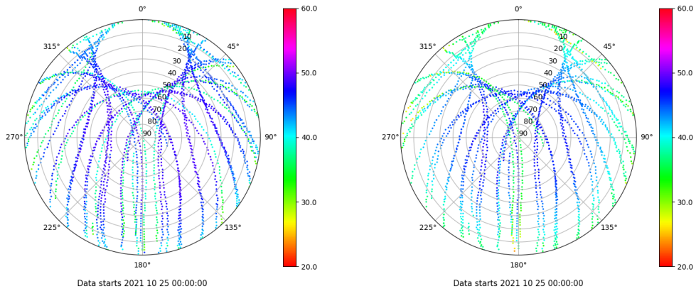
Skyplot for station VALE. Signal to Noise S1C Data file VALE00ESP_R_2021298.xtr Skyplot for station VALE. Signal to Noise S2P Data file VALE00ESP_R_2021298.xtr
