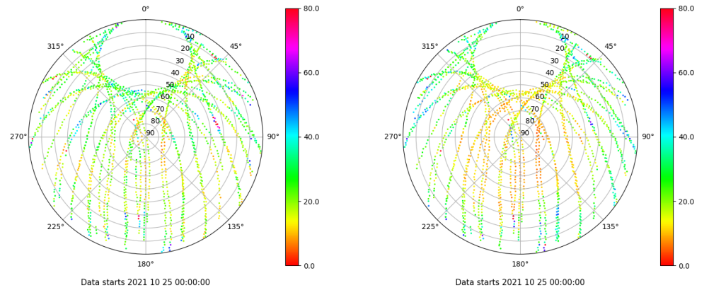
Skyplot for station VALE. Parameter M1C Data file VALE00ESP_R_2021298.xtr Skyplot for station VALE. Parameter M2P Data file VALE00ESP_R_2021298.xtr
