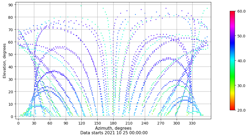
Azimuth-elevation plot for station VALE. Signal to Noise S1C Data file VALE00ESP_R_2021298.xtr
