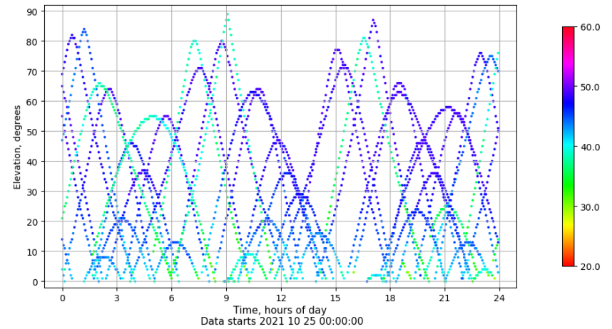
Time-elevation plot for station VALE. Signal to Noise S1C Data file VALE00ESP_R_2021298.xtr
