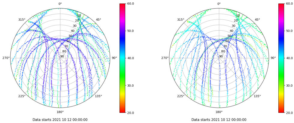
Skyplot for station VALE. Signal to Noise S1C Data file VALE00ESP_R_2021285.xtr Skyplot for station VALE. Signal to Noise S2P Data file VALE00ESP_R_2021285.xtr
