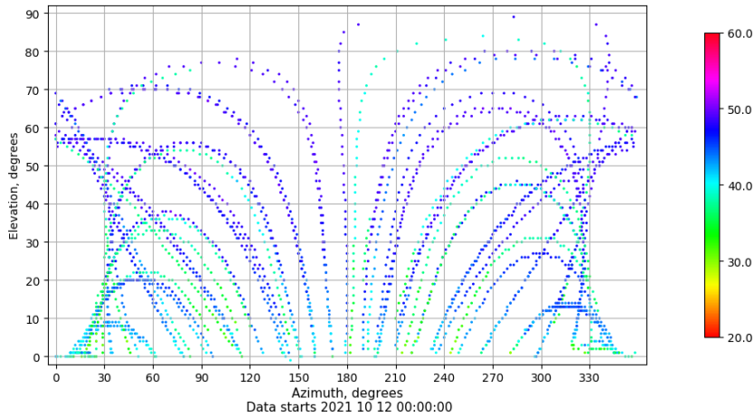
Azimuth-elevation plot for station VALE. Signal to Noise S1C Data file VALE00ESP_R_2021285.xtr
