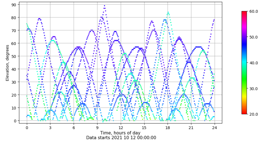
Time-elevation plot for station VALE. Signal to Noise S1C Data file VALE00ESP_R_2021285.xtr
