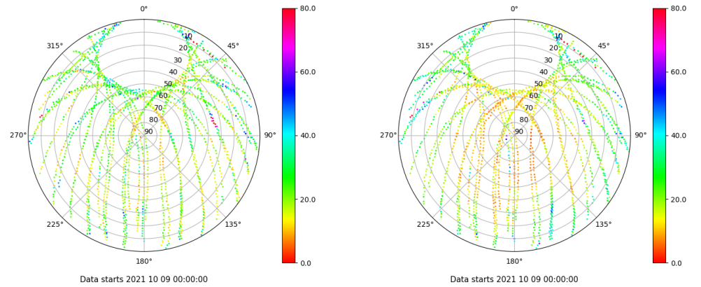
Skyplot for station VALE. Parameter M1C Data file VALE00ESP_R_2021282.xtr Skyplot for station VALE. Parameter M2P Data file VALE00ESP_R_2021282.xtr
