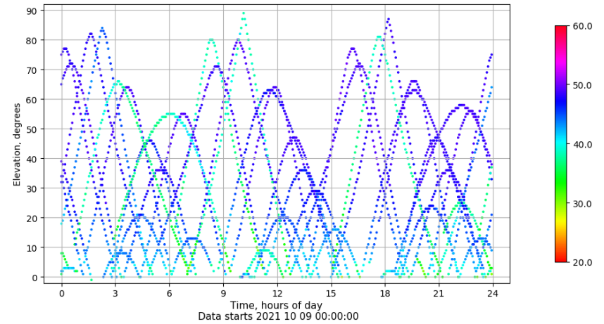
Time-elevation plot for station VALE. Signal to Noise S1C Data file VALE00ESP_R_2021282.xtr
