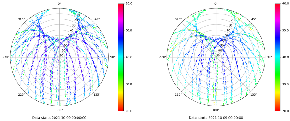
Skyplot for station VALE. Signal to Noise S1C Data file VALE00ESP_R_2021282.xtr Skyplot for station VALE. Signal to Noise S2P Data file VALE00ESP_R_2021282.xtr
