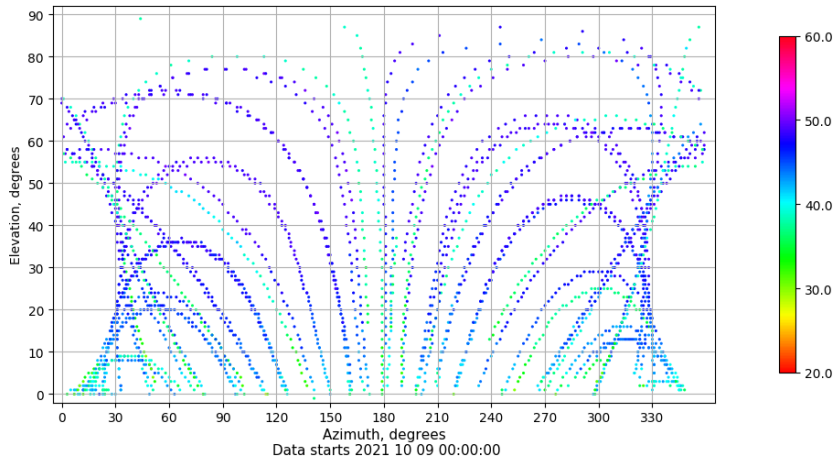
Azimuth-elevation plot for station VALE. Signal to Noise S1C Data file VALE00ESP_R_2021282.xtr
