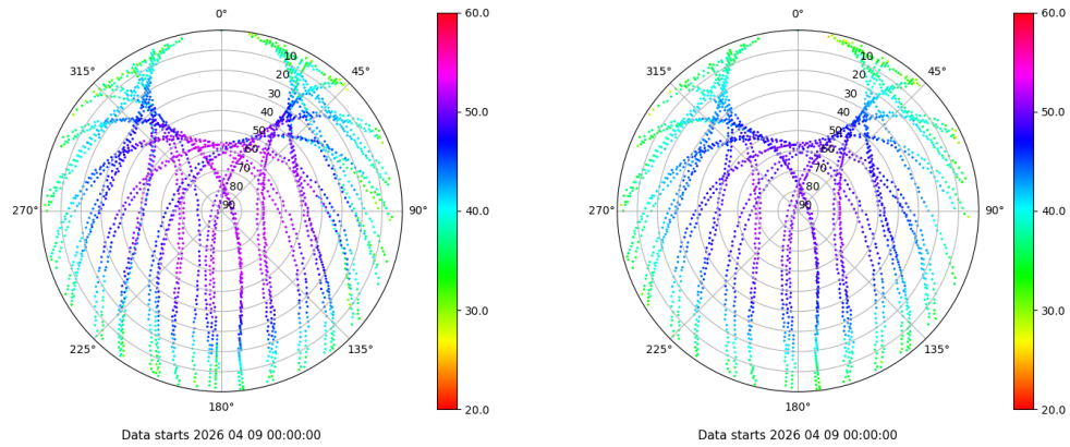
Skyplot for station VALC. Signal to Noise S1C Data file VALC00ESP_R_2026099.xtr Skyplot for station VALC. Signal to Noise S2C Data file VALC00ESP_R_2026099.xtr
