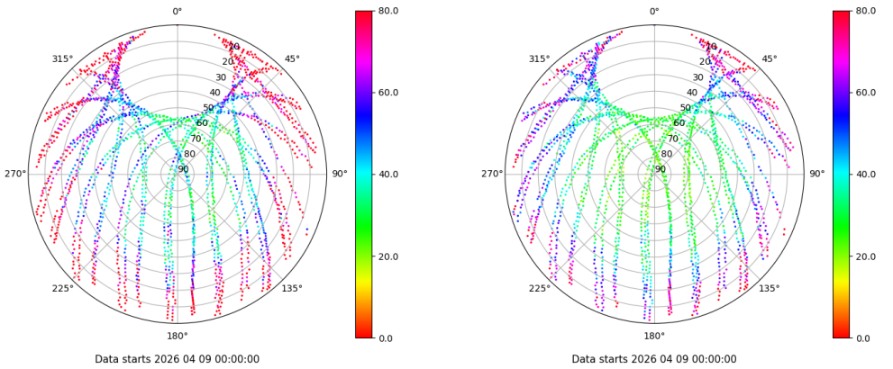
Skyplot for station VALC. Parameter M1C Data file VALC00ESP_R_2026099.xtr Skyplot for station VALC. Parameter M2C Data file VALC00ESP_R_2026099.xtr
