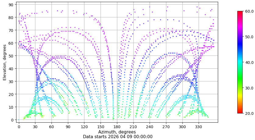
Azimuth-elevation plot for station VALC. Signal to Noise S1C Data file VALC00ESP_R_2026099.xtr
