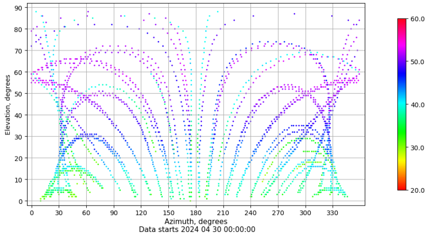
Azimuth-elevation plot for station VALC. Signal to Noise S1C Data file VALC00ESP_R_2024121.xtr
