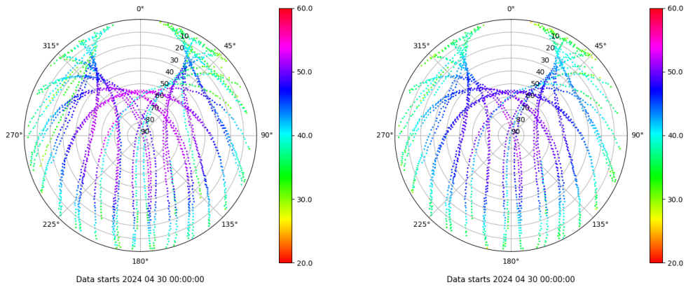
Skyplot for station VALC. Signal to Noise S1C Data file VALC00ESP_R_2024121.xtr Skyplot for station VALC. Signal to Noise S2C Data file VALC00ESP_R_2024121.xtr
