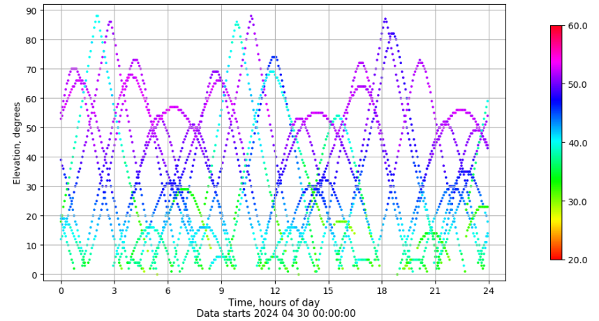
Time-elevation plot for station VALC. Signal to Noise S1C Data file VALC00ESP_R_2024121.xtr
