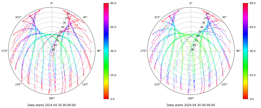
Skyplot for station VALC. Parameter M1C Data file VALC00ESP_R_2024121.xtr Skyplot for station VALC. Parameter M2C Data file VALC00ESP_R_2024121.xtr
