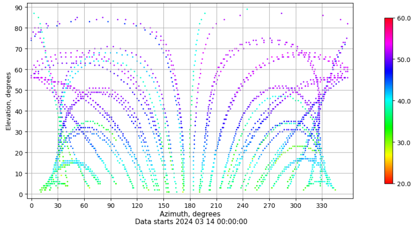
Azimuth-elevation plot for station VALC. Signal to Noise S1C Data file VALC00ESP_R_2024074.xtr
