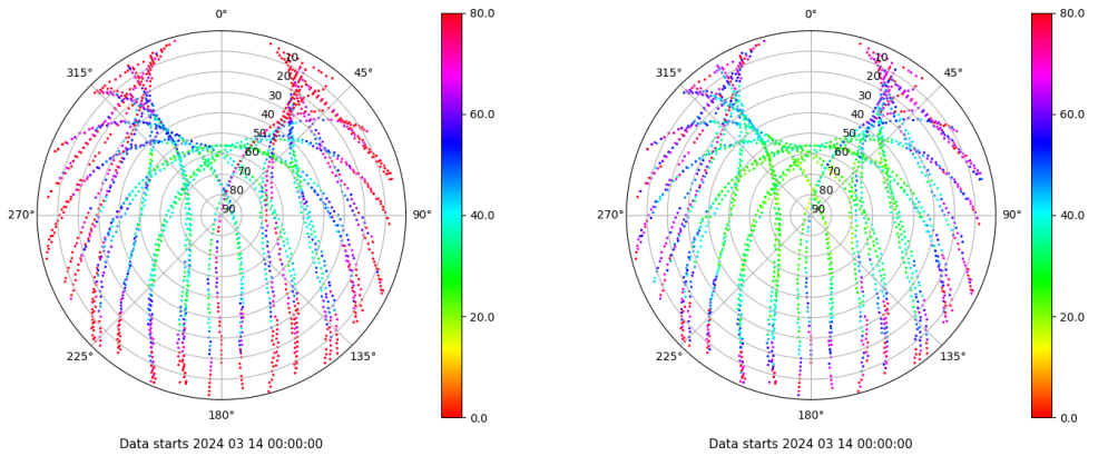
Skyplot for station VALC. Parameter M1C Data file VALC00ESP_R_2024074.xtr Skyplot for station VALC. Parameter M2C Data file VALC00ESP_R_2024074.xtr
