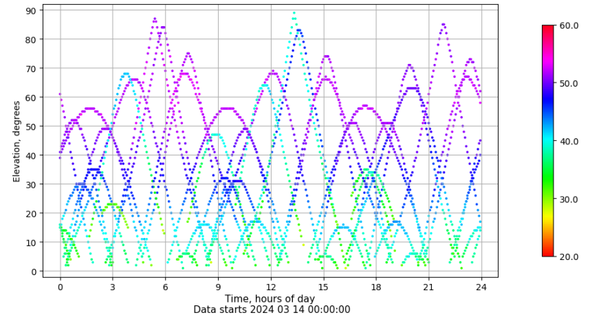
Time-elevation plot for station VALC. Signal to Noise S1C Data file VALC00ESP_R_2024074.xtr
