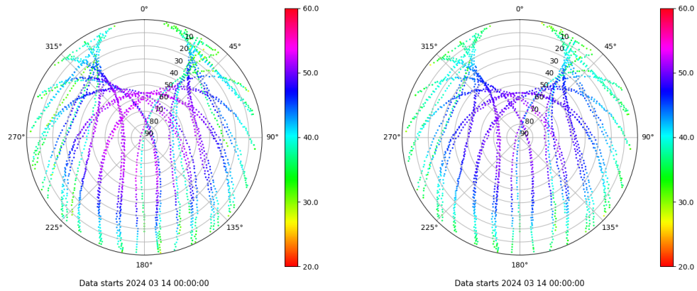
Skyplot for station VALC. Signal to Noise S1C Data file VALC00ESP_R_2024074.xtr Skyplot for station VALC. Signal to Noise S2C Data file VALC00ESP_R_2024074.xtr
