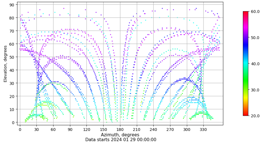
Azimuth-elevation plot for station VALC. Signal to Noise S1C Data file VALC00ESP_R_2024029.xtr
