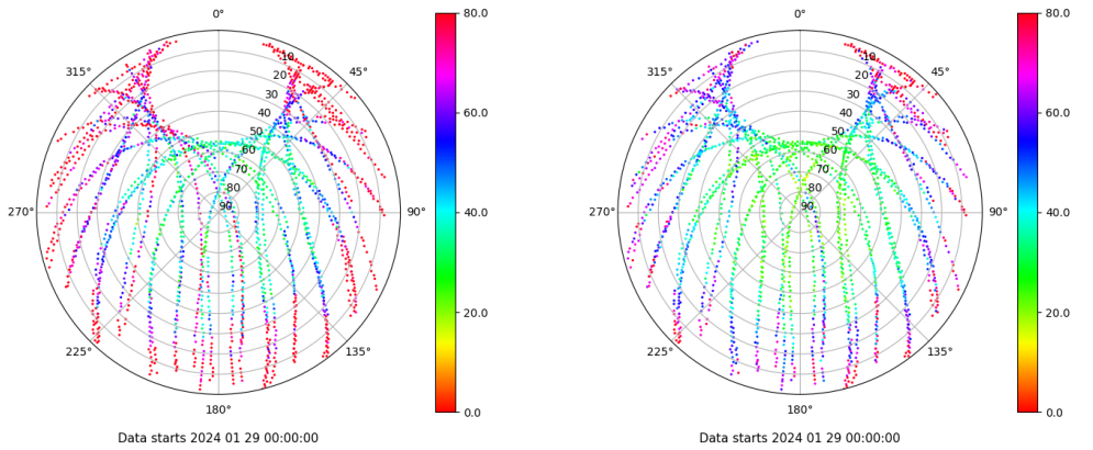
Skyplot for station VALC. Parameter M1C Data file VALC00ESP_R_2024029.xtr Skyplot for station VALC. Parameter M2C Data file VALC00ESP_R_2024029.xtr
