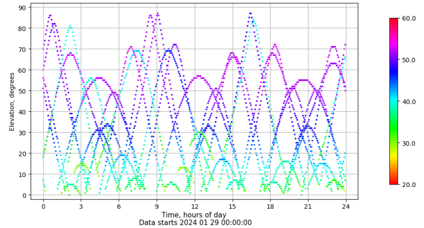
Time-elevation plot for station VALC. Signal to Noise S1C Data file VALC00ESP_R_2024029.xtr
