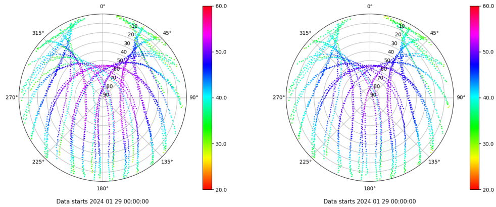
Skyplot for station VALC. Signal to Noise S1C Data file VALC00ESP_R_2024029.xtr Skyplot for station VALC. Signal to Noise S2C Data file VALC00ESP_R_2024029.xtr
