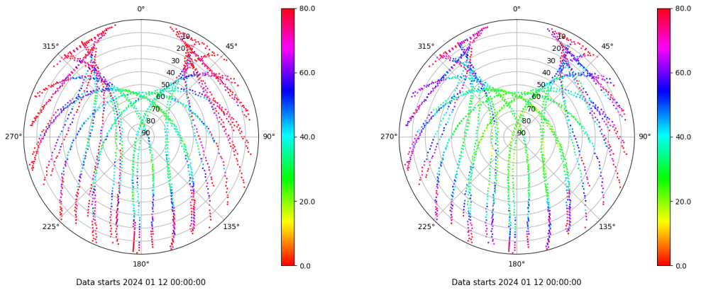
Skyplot for station VALC. Parameter M1C Data file VALC00ESP_R_2024012.xtr Skyplot for station VALC. Parameter M2C Data file VALC00ESP_R_2024012.xtr
