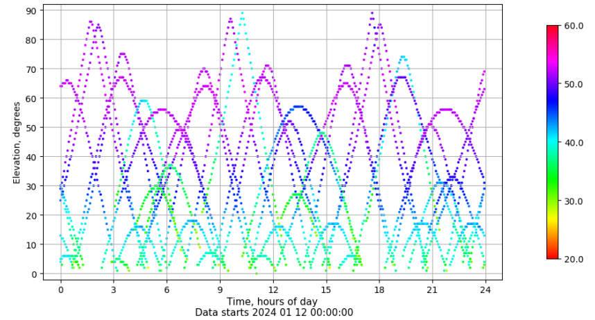
Time-elevation plot for station VALC. Signal to Noise S1C Data file VALC00ESP_R_2024012.xtr
