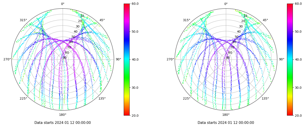
Skyplot for station VALC. Signal to Noise S1C Data file VALC00ESP_R_2024012.xtr Skyplot for station VALC. Signal to Noise S2C Data file VALC00ESP_R_2024012.xtr
