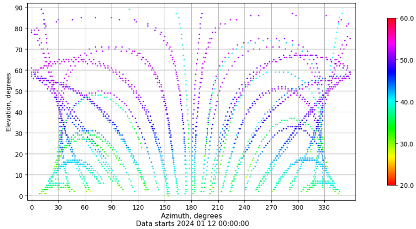
Azimuth-elevation plot for station VALC. Signal to Noise S1C Data file VALC00ESP_R_2024012.xtr
