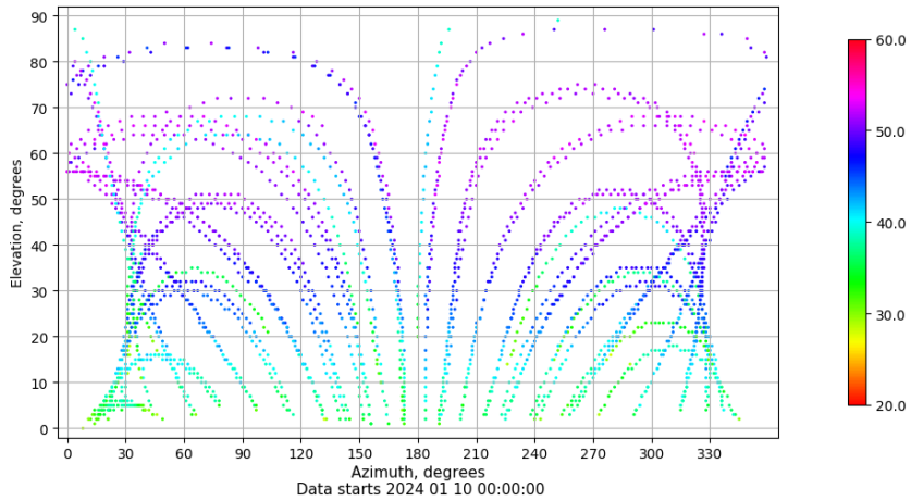
Azimuth-elevation plot for station VALC. Signal to Noise S1C Data file VALC00ESP_R_2024010.xtr
