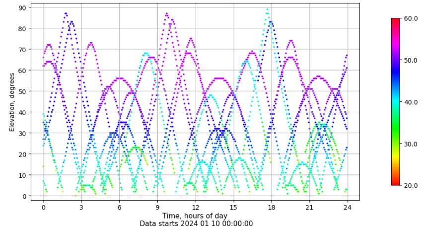
Time-elevation plot for station VALC. Signal to Noise S1C Data file VALC00ESP_R_2024010.xtr
