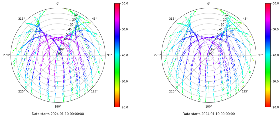
Skyplot for station VALC. Signal to Noise S1C Data file VALC00ESP_R_2024010.xtr Skyplot for station VALC. Signal to Noise S2C Data file VALC00ESP_R_2024010.xtr
