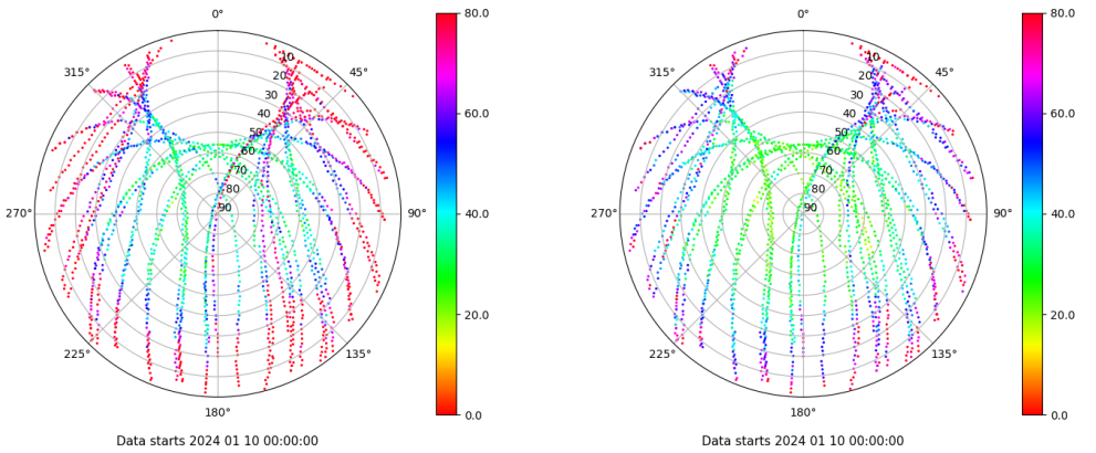
Skyplot for station VALC. Parameter M1C Data file VALC00ESP_R_2024010.xtr Skyplot for station VALC. Parameter M2C Data file VALC00ESP_R_2024010.xtr
