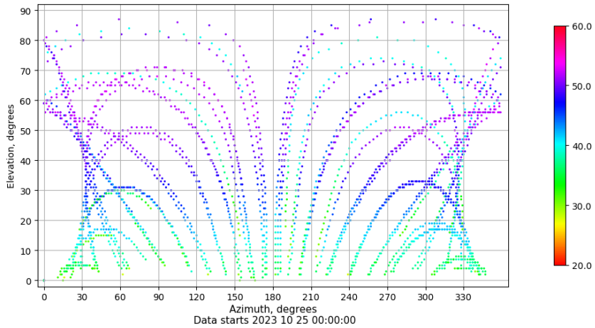
Azimuth-elevation plot for station VALC. Signal to Noise S1C Data file VALC00ESP_R_2023298.xtr
