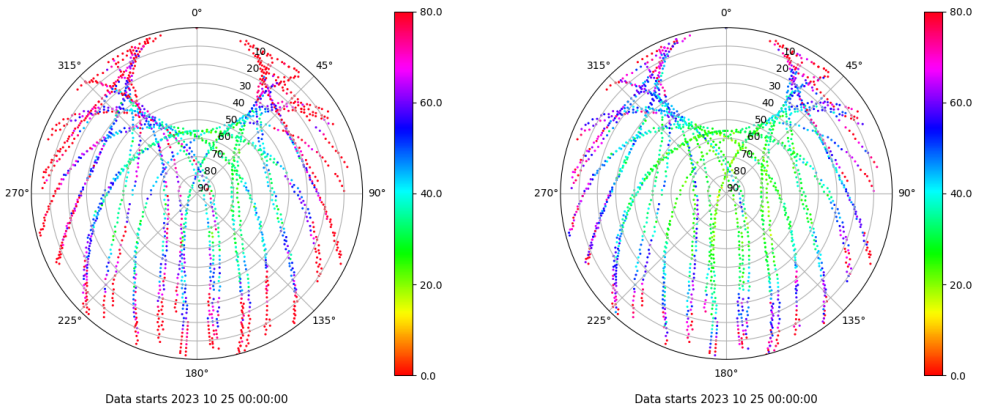
Skyplot for station VALC. Parameter M1C Data file VALC00ESP_R_2023298.xtr Skyplot for station VALC. Parameter M2C Data file VALC00ESP_R_2023298.xtr
