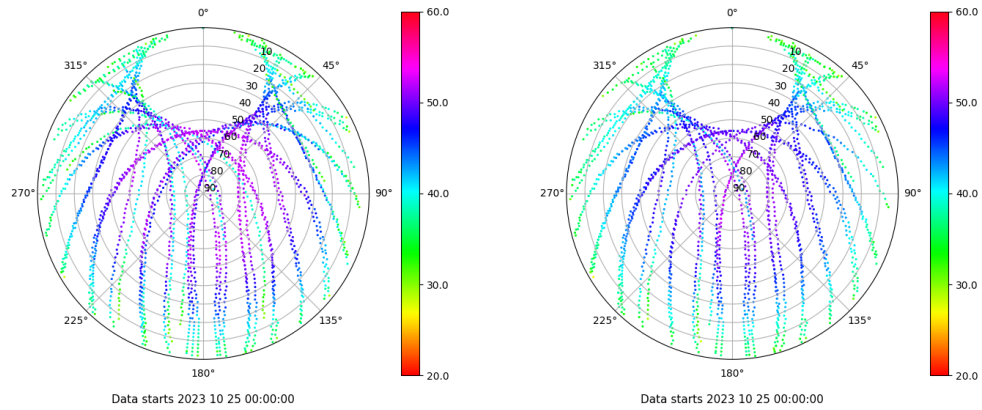
Skyplot for station VALC. Signal to Noise S1C Data file VALC00ESP_R_2023298.xtr Skyplot for station VALC. Signal to Noise S2C Data file VALC00ESP_R_2023298.xtr
