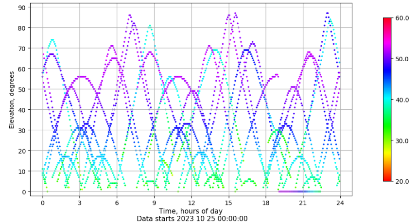
Time-elevation plot for station VALC. Signal to Noise S1C Data file VALC00ESP_R_2023298.xtr
