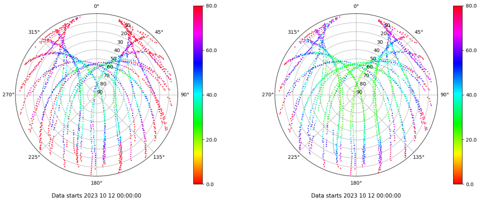
Skyplot for station VALC. Parameter M1C Data file VALC00ESP_R_2023285.xtr Skyplot for station VALC. Parameter M2C Data file VALC00ESP_R_2023285.xtr
