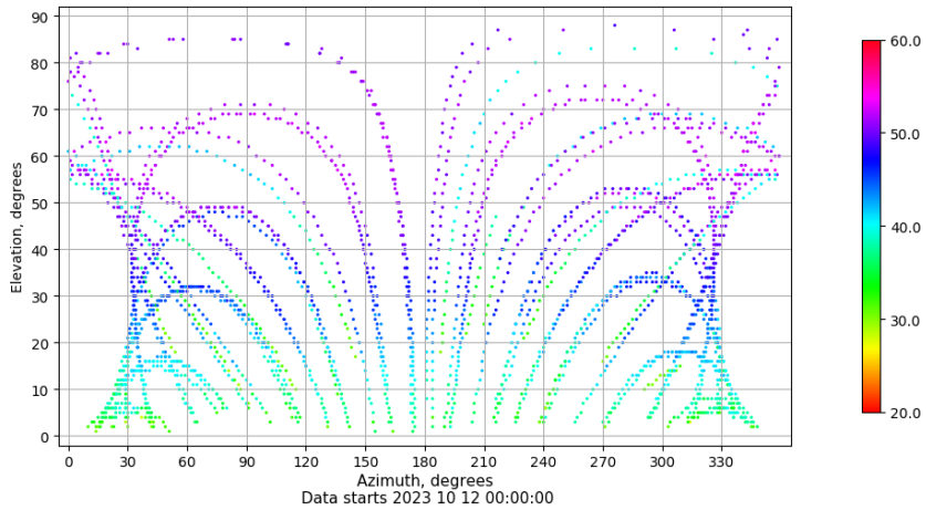
Azimuth-elevation plot for station VALC. Signal to Noise S1C Data file VALC00ESP_R_2023285.xtr
