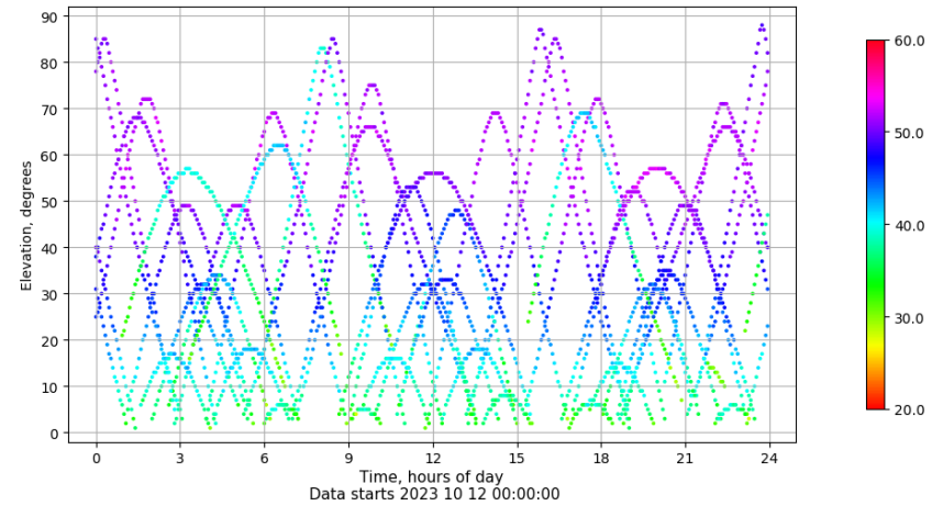
Time-elevation plot for station VALC. Signal to Noise S1C Data file VALC00ESP_R_2023285.xtr
