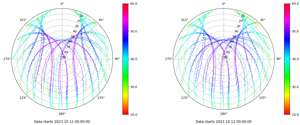
Skyplot for station VALC. Signal to Noise S1C Data file VALC00ESP_R_2023285.xtr Skyplot for station VALC. Signal to Noise S2C Data file VALC00ESP_R_2023285.xtr
