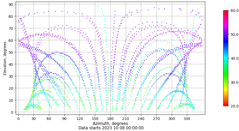
Azimuth-elevation plot for station VALC. Signal to Noise S1C Data file VALC00ESP_R_2023281.xtr
