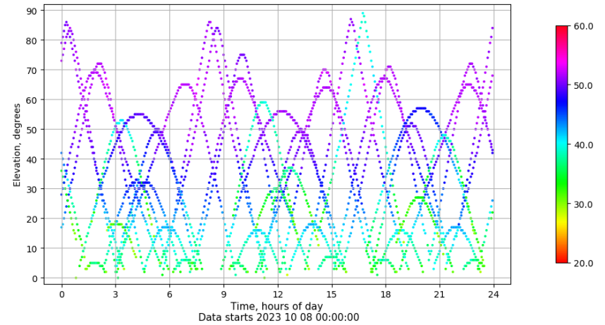
Time-elevation plot for station VALC. Signal to Noise S1C Data file VALC00ESP_R_2023281.xtr
