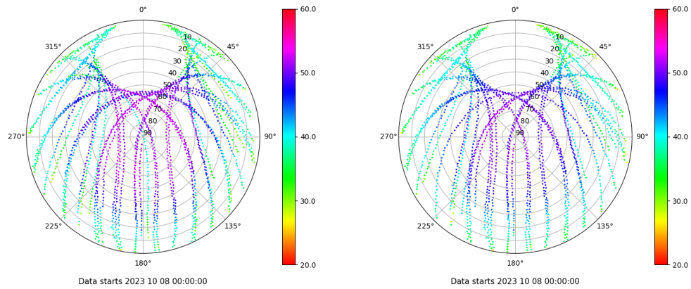
Skyplot for station VALC. Signal to Noise S1C Data file VALC00ESP_R_2023281.xtr Skyplot for station VALC. Signal to Noise S2C Data file VALC00ESP_R_2023281.xtr
