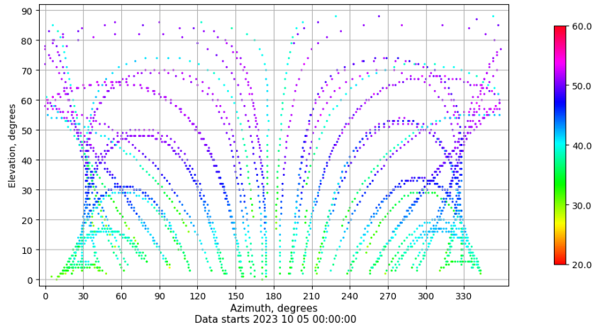
Azimuth-elevation plot for station VALC. Signal to Noise S1C Data file VALC00ESP_R_2023278.xtr
