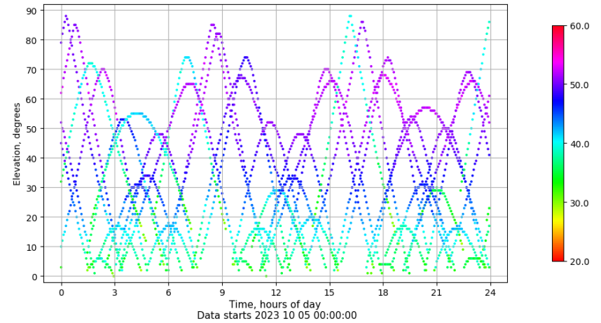
Time-elevation plot for station VALC. Signal to Noise S1C Data file VALC00ESP_R_2023278.xtr
