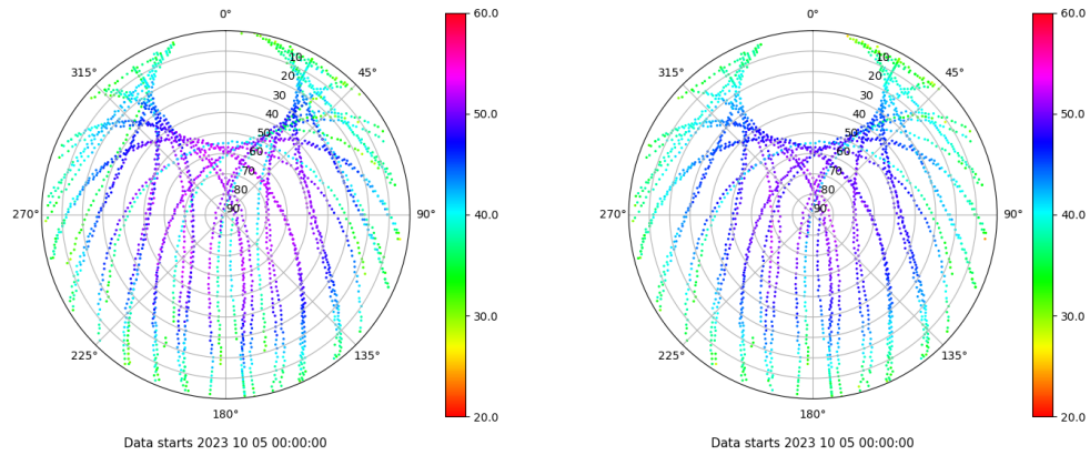
Skyplot for station VALC. Signal to Noise S1C Data file VALC00ESP_R_2023278.xtr Skyplot for station VALC. Signal to Noise S2C Data file VALC00ESP_R_2023278.xtr
