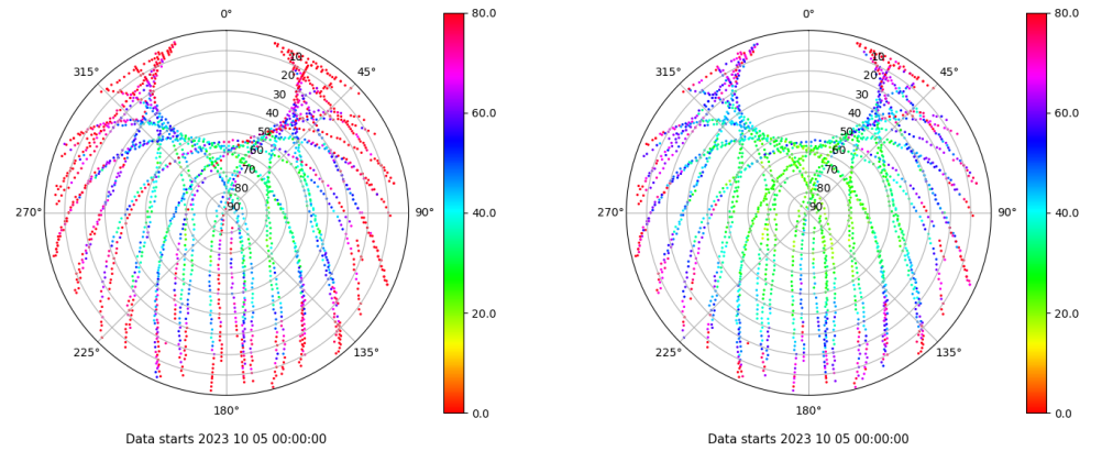
Skyplot for station VALC. Parameter M1C Data file VALC00ESP_R_2023278.xtr Skyplot for station VALC. Parameter M2C Data file VALC00ESP_R_2023278.xtr
