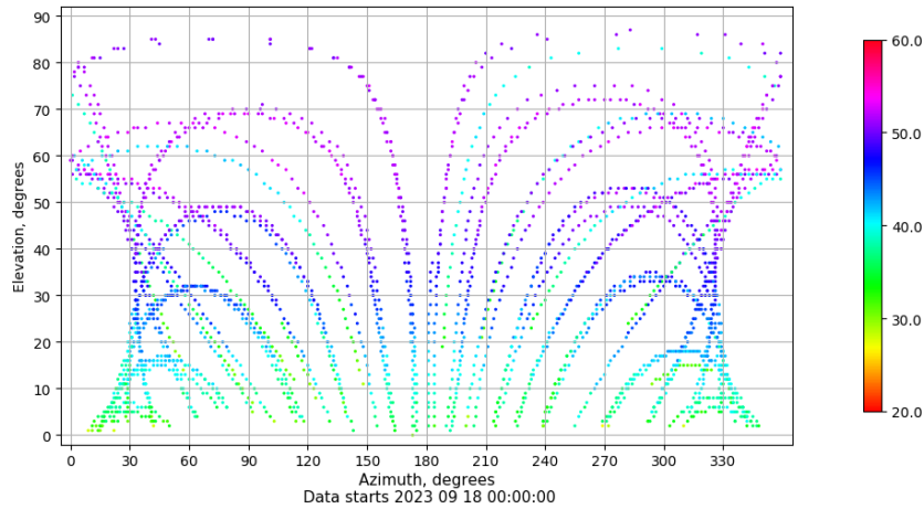
Azimuth-elevation plot for station VALC. Signal to Noise S1C Data file VALC00ESP_R_2023261.xtr
