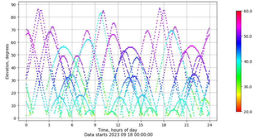
Time-elevation plot for station VALC. Signal to Noise S1C Data file VALC00ESP_R_2023261.xtr
