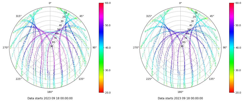
Skyplot for station VALC. Signal to Noise S1C Data file VALC00ESP_R_2023261.xtr Skyplot for station VALC. Signal to Noise S2C Data file VALC00ESP_R_2023261.xtr
