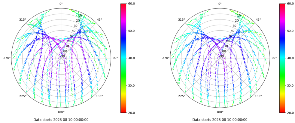
Skyplot for station VALC. Signal to Noise S1C Data file VALC00ESP_R_2023222.xtr Skyplot for station VALC. Signal to Noise S2C Data file VALC00ESP_R_2023222.xtr
