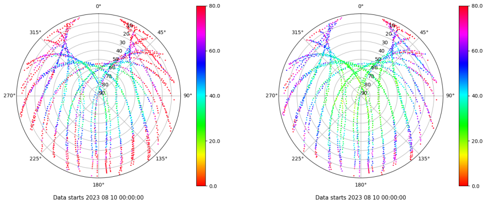
Skyplot for station VALC. Parameter M1C Data file VALC00ESP_R_2023222.xtr Skyplot for station VALC. Parameter M2C Data file VALC00ESP_R_2023222.xtr
