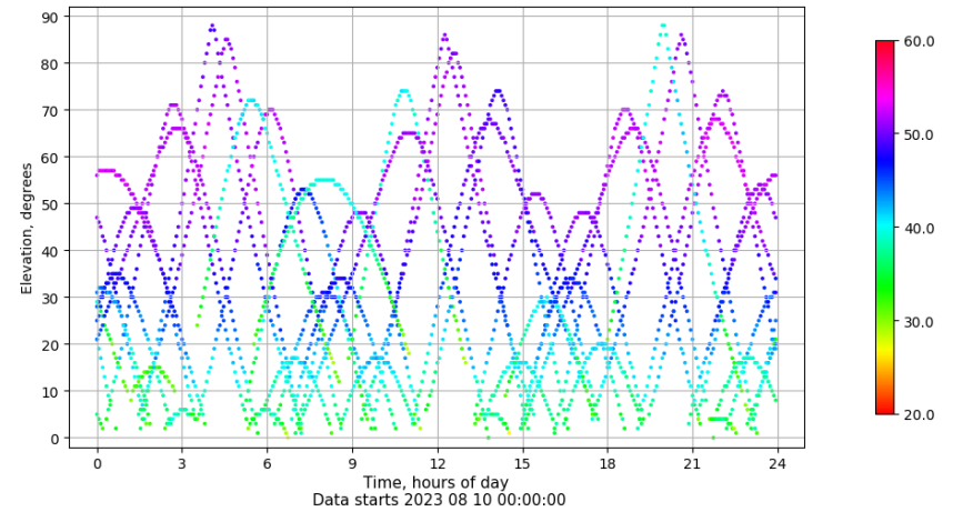
Time-elevation plot for station VALC. Signal to Noise S1C Data file VALC00ESP_R_2023222.xtr
