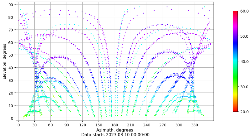
Azimuth-elevation plot for station VALC. Signal to Noise S1C Data file VALC00ESP_R_2023222.xtr
