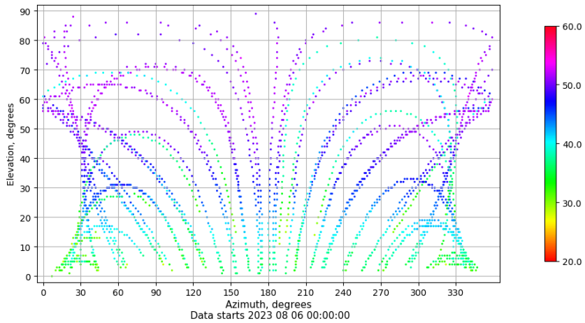
Azimuth-elevation plot for station VALC. Signal to Noise S1C Data file VALC00ESP_R_2023218.xtr
