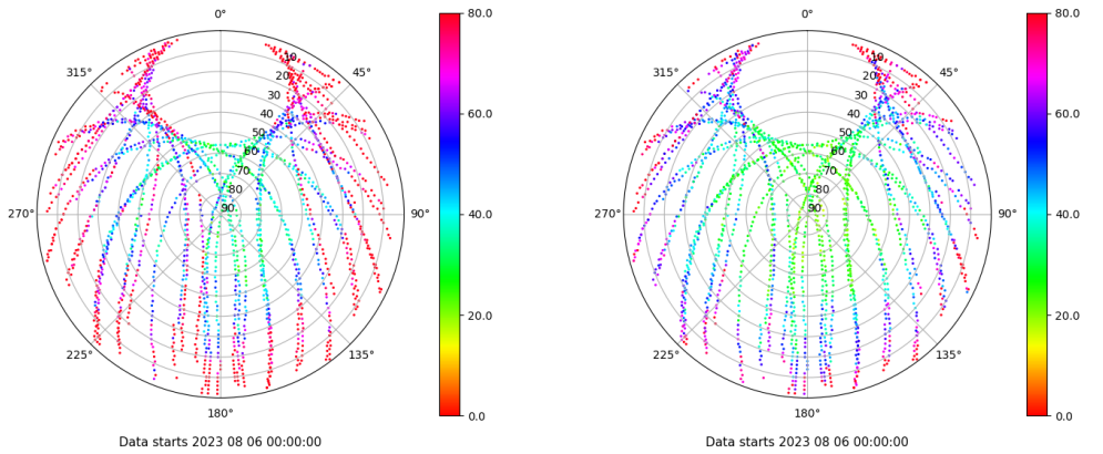
Skyplot for station VALC. Parameter M1C Data file VALC00ESP_R_2023218.xtr Skyplot for station VALC. Parameter M2C Data file VALC00ESP_R_2023218.xtr
