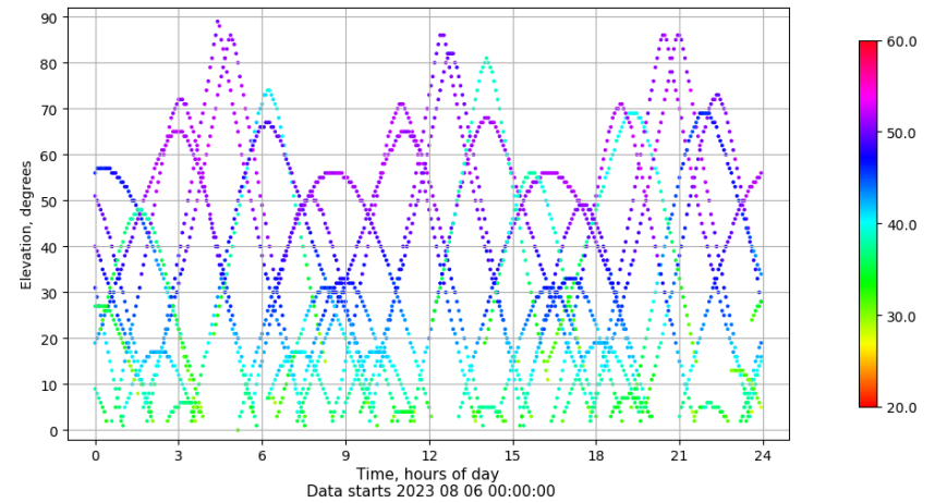
Time-elevation plot for station VALC. Signal to Noise S1C Data file VALC00ESP_R_2023218.xtr
