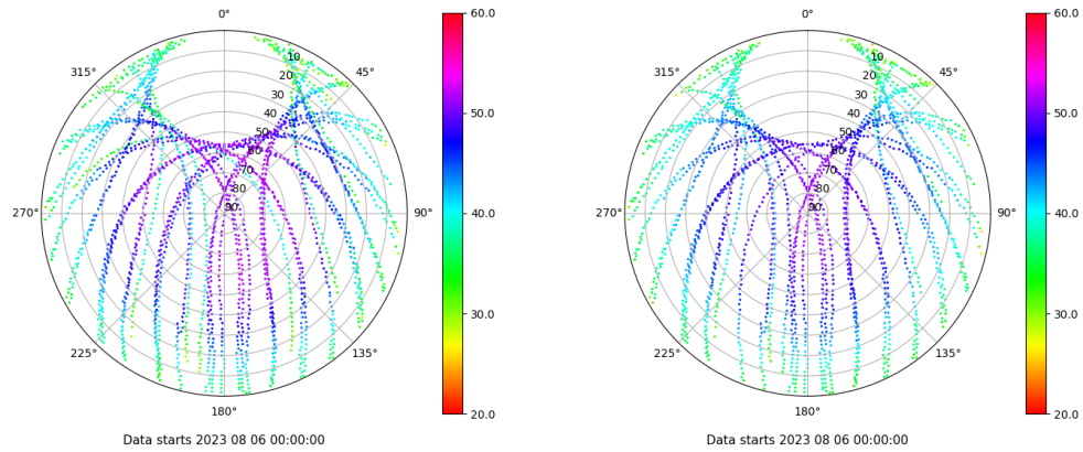
Skyplot for station VALC. Signal to Noise S1C Data file VALC00ESP_R_2023218.xtr Skyplot for station VALC. Signal to Noise S2C Data file VALC00ESP_R_2023218.xtr
